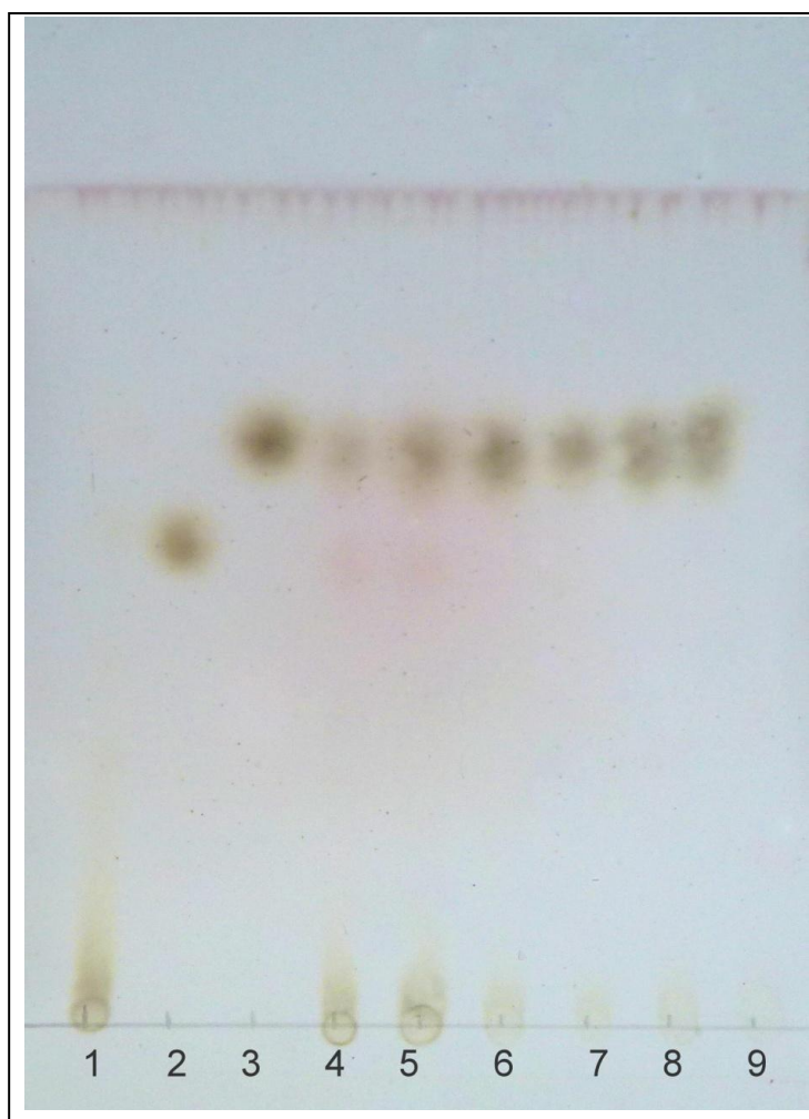
Fig. 7 TLC chromatogram of the products of hydrolysis of inulin with inulinase from A. kawachii . Lane 1: inulin standard, Lane 2: sucrose standard, Lane 3: fructose standard, Lanes 4-9: hydrolysis products of inulin by inulinase (reaction times from 1 to 6 hrs). Sample volume: 5 \mu . TLC plates were developed twice with n-butanol-isopropanol-acetic acid-water (7:5:4:2) as the developing solvent in ascending TLC.
