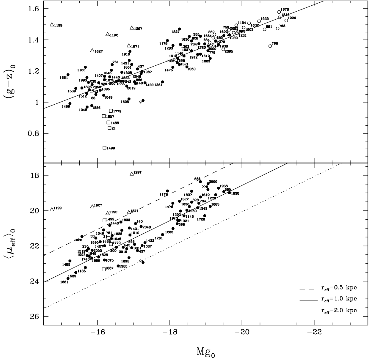
Fig. 2.— Distance, extinction and reddening corrected color–magnitude ( top ) and \langle \mu_{\text{eff}} \rangle –magnitude ( bottom ) diagrams of the galaxies included in the ACSVCS, built from our photometry. The numbers correspond to the VCC designation of each galaxy. In the top panel, we depict with open circles incomplete galaxies, not shown in the bottom panel as we were not able to estimate their r_{\text{eff}} . With open triangles we show the objects consistent with being cE galaxies, and with open squares those that show blue centers and evidence of recent star formation. The dashed line in the top panel represents the linear fit to the CMR when incomplete galaxies, cEs and dwarfs with evidence of recent star formation are excluded from the sample. The different lines shown in the bottom panel depict loci of constant r_{\text{eff}} .
