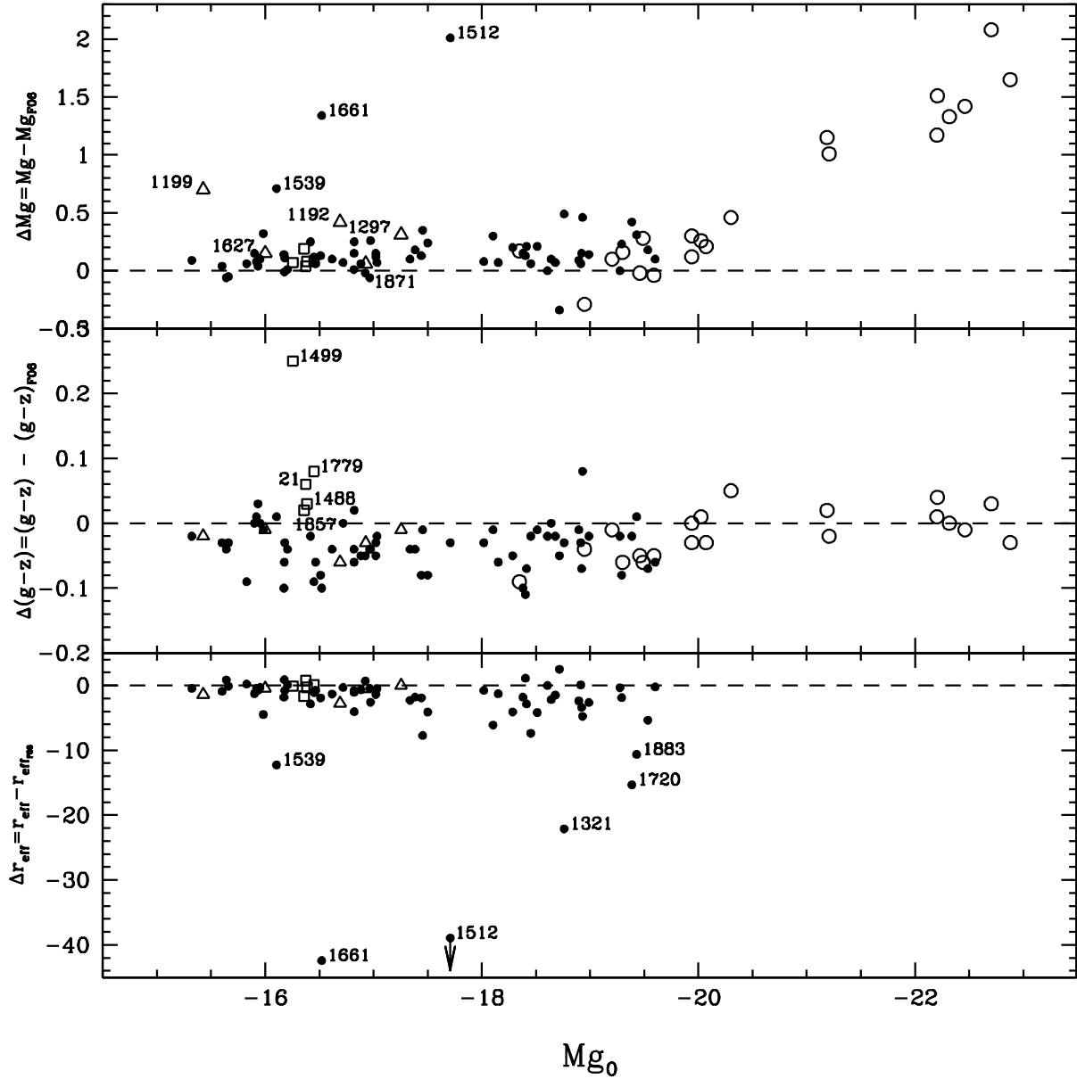
Fig. 4.— We show the differences between our g magnitudes ( top ), (g - z) colors ( center ) and r_{\text{eff}} values in arcsec ( bottom ), and those reported by F06 for the galaxies of the ACSVCS. We depict with open circles incomplete galaxies. For clarity, in the top plot we only label the cE galaxies ( open triangles ) and in the centered one, the blue galaxies ( open squares ). In all the plots we also label the most discrepant galaxies that are complete within the ACS frames.
