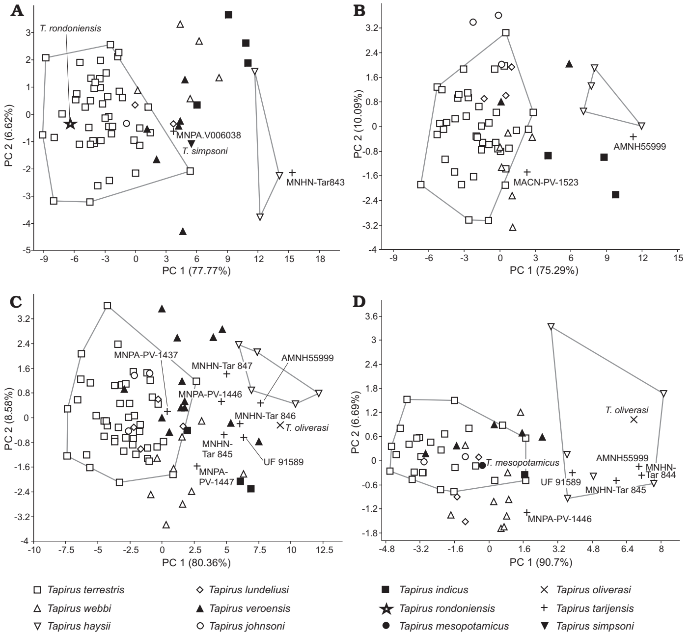
Fig. 6. Principal Component analyses including Tapirus terrestris , T. webbi , T. haysii , T. lundeliusi , T. veroensis , T. johnsoni , T. indicus , T. rondoniensi , T. mesopotamicus , T. oliverasi , T. tarijensis , and T. simpsoni . A . Upper dentition (Pm2, M1–M2). B . Lower dentition (pm2–pm4). C . Lower dentition (m1–m2). D . Lower dentition (m3).
