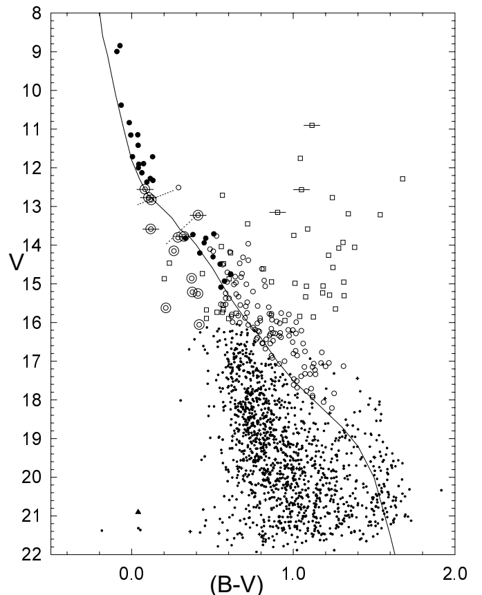
Fig. 5. Colour-magnitude diagram (CMD) [ V vs. (B - V) ] of stars in the field of NGC 2571. Symbols as in Fig. 4. The solid line represents the Schmidt-Kaler (1982) ZAMS. The dotted lines show the position of the gap (see Sect. 3.7).
