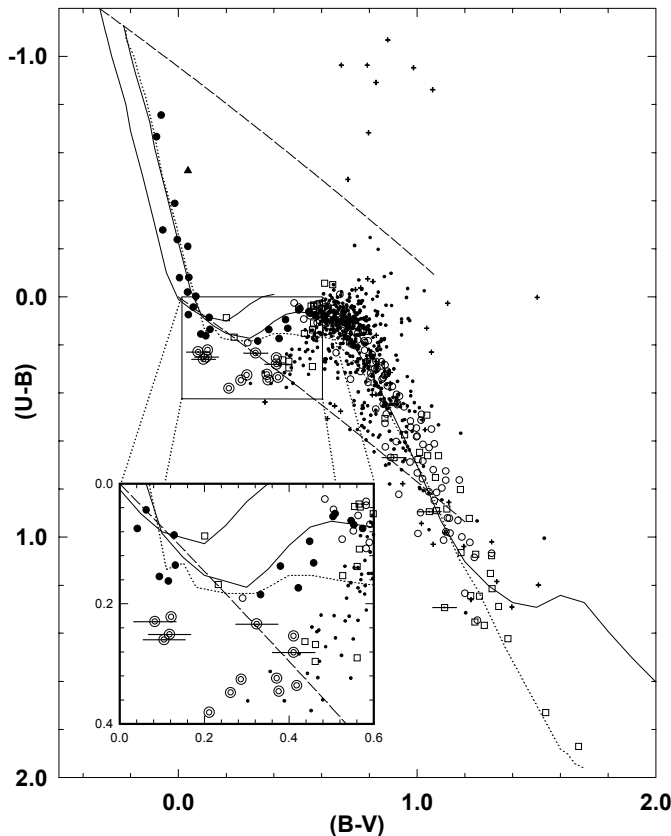
Fig. 4. Two-colour diagram (TCD) [ (U - B) vs. (B - V) ] of stars in the field of NGC 2571. Symbols are: \bullet bright cluster members; \circ fainter cluster members up to 1 mag above the ZAMS; \square non-members; \cdot distant field stars; + stars with large photometric errors; double circles: probable metallic line stars; symbols with horizontal bar: variable stars; black triangle: probable white-dwarf. – The relation for luminosity class V from Schmidt-Kaler (1982) is shown twice (solid lines): first, unshifted (in the upper left part), and second, shifted by E_{(B-V)} = 0.1 along the standard reddening path (dashed lines). The dotted line is the relation for giant stars. – Insert: magnification of the lower left part of the TCD.
