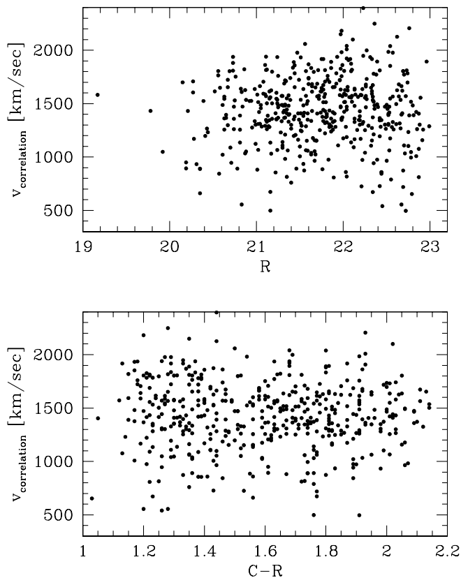
FIG. 8.—Luminosity ( top ) and color ( bottom ) dependence of the correlation velocities. No correlation is seen with luminosity; however, the scatter of blue objects is larger than that of red objects, which is due to their different dynamics explained in Paper II.
