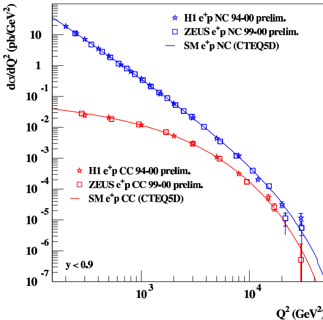
FIG. 5: Electroweak unification
