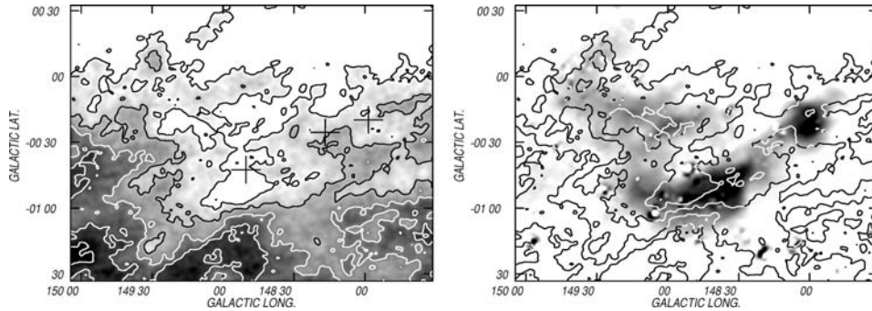
Figure 7. (a) H I emission distribution for the structure probably related to SH 148.83–0.67 within the velocity range -25.0 to -28.0 \text{km s}^{-1} . The grey-scale is from 60 to 100 K. The contour levels are 60 to 100 K in steps of 10 K. The crosses indicate the positions of HD 24431, ALS 773, and HD 24094. (b) Overlay of the H I emission distribution (contour lines) and the VTSS image (grey-scale). Darker regions mean brighter areas.
