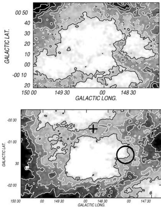
Figure 8. (a) H I emission distribution for the neutral atomic gas structure probably related to SH 149.25–0.0 within the velocity range -13.4 to -16.7 \text{km s}^{-1} . The grey-scale is 15 to 45 K. The contour levels are 10, and from 20 to 50 K in steps of 5 K. (b) H I emission distribution within the velocity interval from -3.1 to -17.1 \text{km s}^{-1} showing the H I structure at (l, b) = (149^\circ 0', -1^\circ 30') . The contour levels are from 50 to 65 K in steps of 5 K. The positions of HD 24431 and NGC 1444 are indicated by a cross and a circle, respectively. Darker regions mean brighter areas.
