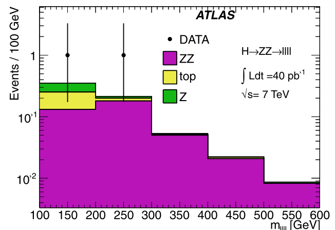
Fig. 5 Distribution of m_{\ell\ell\ell\ell} in the H \rightarrow ZZ^{(*)} \rightarrow \ell\ell\ell\ell search before applying the lepton impact parameter and isolation requirements which remove the two candidates. The error bars reflect Poisson asymmetric errors
