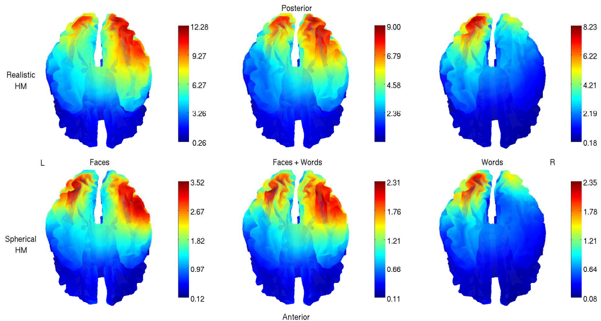
Figure 5. sLORETA source images ( \text{SCDP} \times 10^{-6} ) of N170 component peak for ADHD patients using the realistic head model (upper row) and the spherical head model (lower row) from a basal view. Three different stimuli are depicted: faces (first column), simultaneous faces and words (second column) and words (third column).
