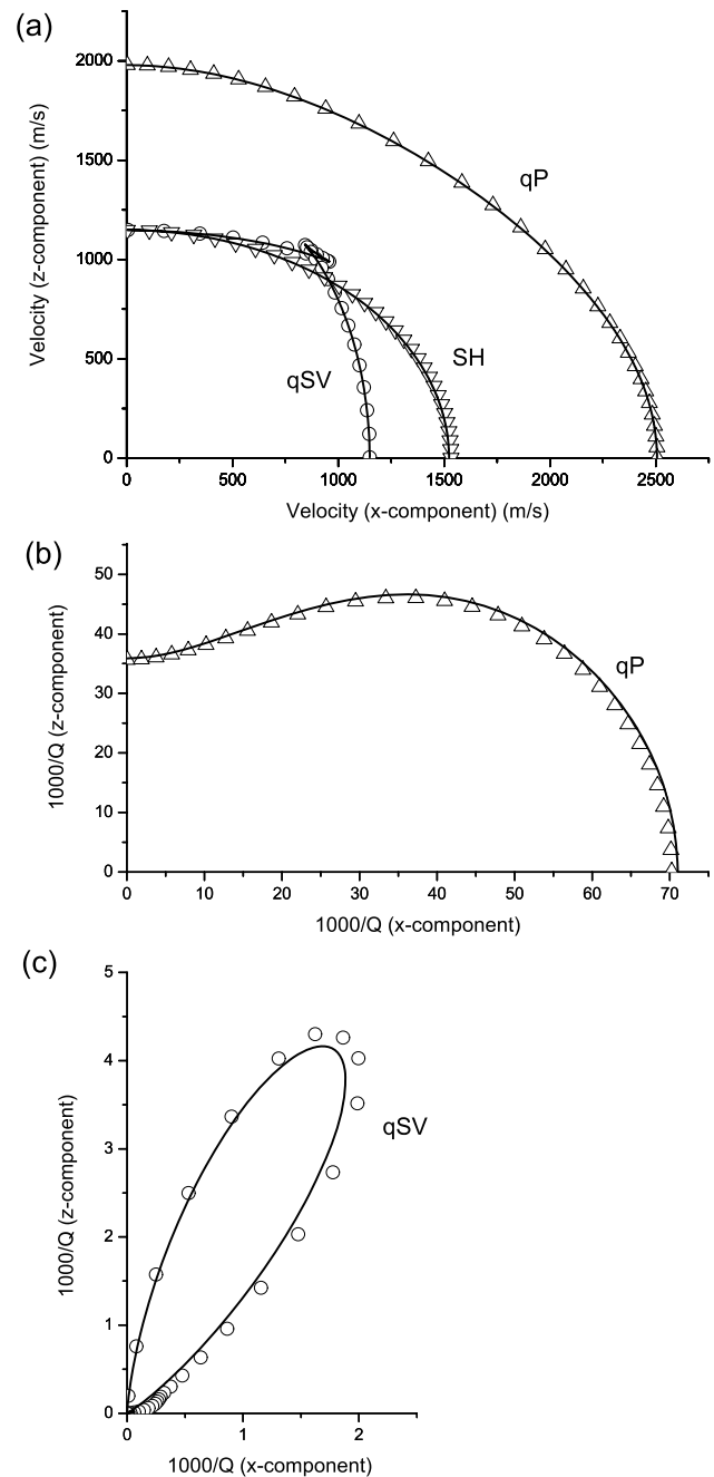
Figure 7. Polar representation of the energy velocity (a) and dissipation factors (b and c) corresponding to a frequency of 50 Hz. The medium consist of a sequence of mudstone and CO 2 -saturated sandstone layers with thicknesses of 5 and 1 cm, respectively (Fig. 6).
