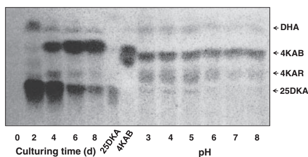
Fig. 2. TLC Chromatogram of 4-Keto-D-arabonate Formation with Ga. liquefaciens .
