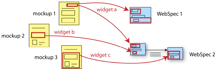
Fig. 4. Overlapping mockups and WebSpec diagrams
