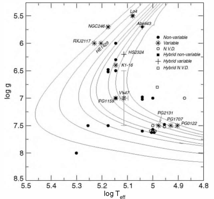
Figure 1. PG1159 evolutionary tracks of Althaus et al. (2005), Miller Bertolami & Althaus (2006), and Córscico et al. (2006), with stellar masses of (from right to left): M_{*} = 0.515, 0.530, 0.542, 0.565, 0.589, 0.609, 0.664, and 0.741 M_{\odot} . Also shown is the location of known PG1159 stars. The error bars for VV 47 are displayed.
