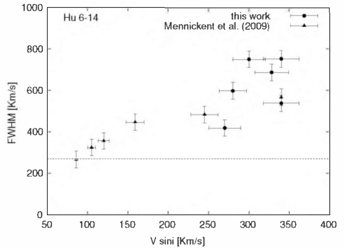
Figure 7. FWHM as a function of V \sin i for Hu_{6-14} . The horizontal line represents the instrumental width.
