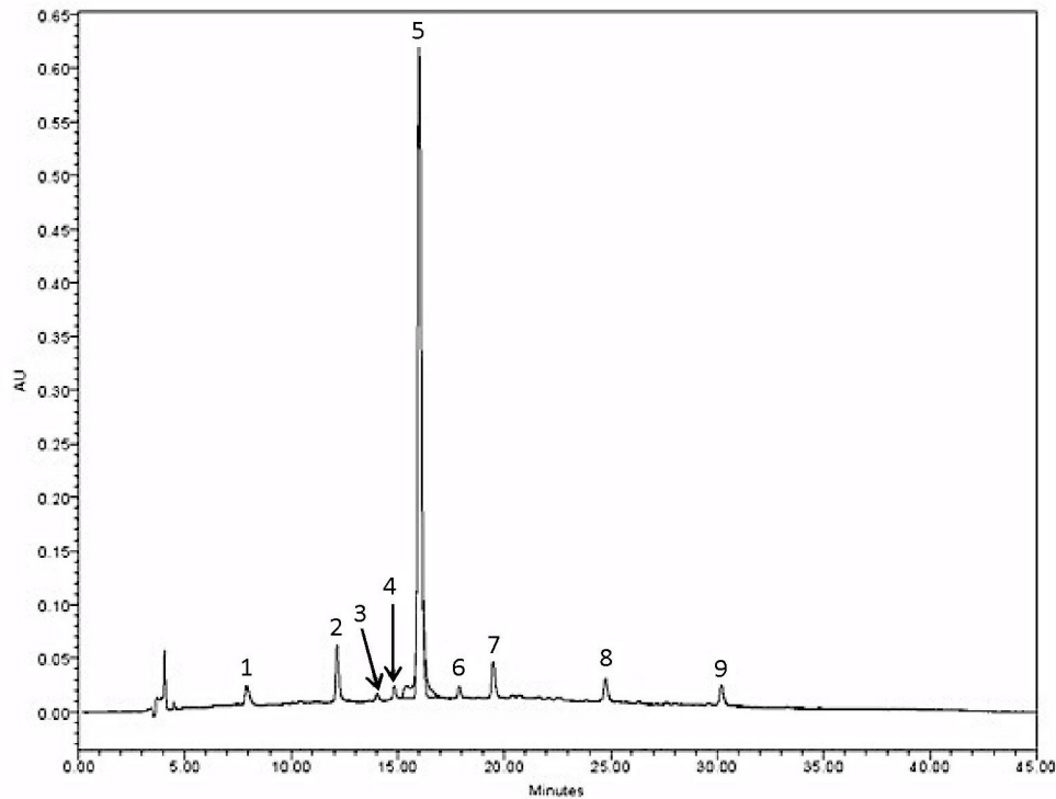
Fig. 1: HPLC chromatogram of anthocyanins in the red wines determined at 520 nm: 1 delphinidin-3-glucoside; 2 cyanidin-3-glucoside; 3 petunidin-3-glucoside; 4 peonidin-3-glucoside; 5 malvidin-3-glucoside; 6 peonidin-3-acetylglucoside; 7 malvidin-3-acetylglucoside; 8 peonidin-3-coumarylglucoside; 9 malvidin-3-coumaroylglucoside.
