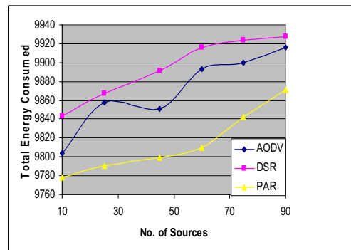
Fig 1 : Total Energy Consumed Vs No. of Sources
