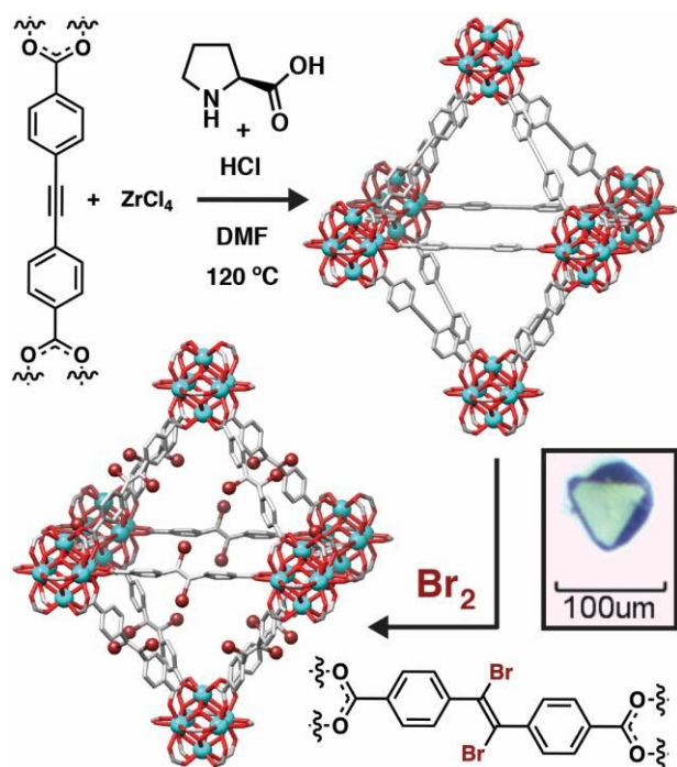
Figure 7. Schematic of L-proline modulated synthesis of a Zr MOF containing the edb linker as single crystals, and its subsequent single-crystal to single-crystal postsynthetic bromination. Reprinted (adapted) with permission from reference 47. Further permissions related to the material should be directed to the American Chemical Society.
