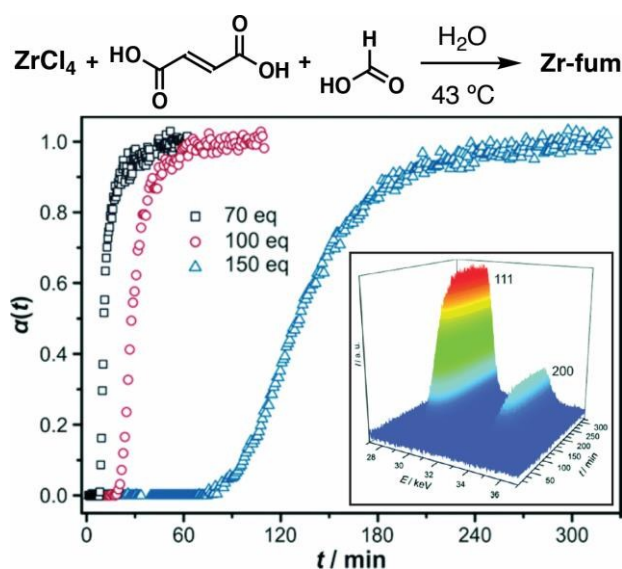
Figure 6. Time evolution of the crystallinity, \alpha , of Zr-fum in aqueous, formic acid modulated syntheses at 43 °C, as assessed by in situ energy-dispersive X-ray diffraction analysis. Inset is a typical 3D plot of diffraction data used to construct \alpha vs t individual curves. Reprinted (adapted) with permission from reference 39. Published (2014) by The Royal Society of Chemistry.
