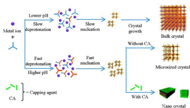
Figure 4. Proposed mechanisms from Zhang et al. to explain the dual roles of pH control and coordination modulation in MOF particle size control. Reprinted with permission from reference 32. Copyright (2012) American Chemical Society.
