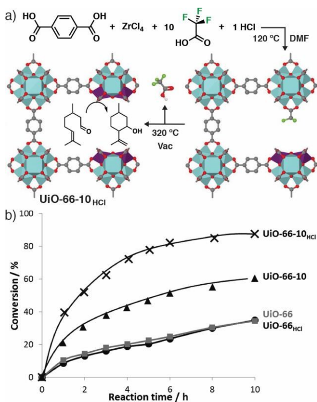
Figure 13. a) Synthesis of a Lewis Acid catalyst based on defective UiO-66, by postsynthetic thermal removal of incorporated trifluoroacetate modulators. b) Enhanced catalytic activity of the TFA-modulated MOFs, UiO-66-10 HCl and UiO-66-10, compared to unmodulated analogues UiO-66 and UiO-66 HCl , in the cyclisation of citronellal. Reprinted with permission from reference 81. Copyright (2013) American Chemical Society.
