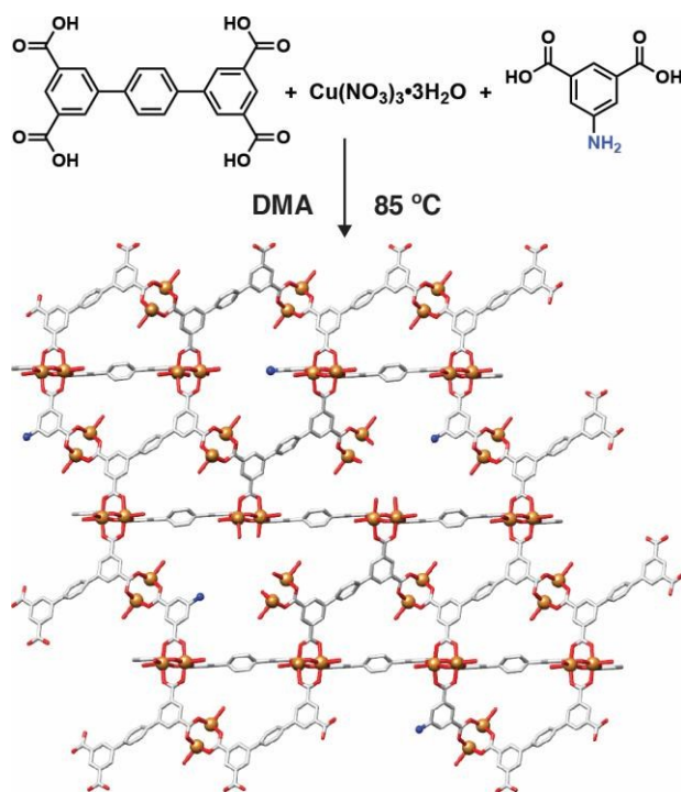
Figure 9. Schematic of 5-aminoisophthalic acid incorporation into NOTT-101 during coordination modulation to modify both pore texture and chemistry through defect formation.
