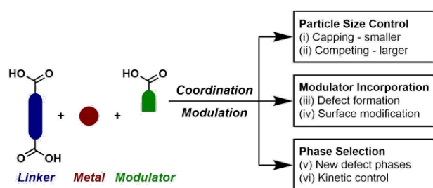
Figure 1. Schematic of coordination modulation, with a range of different potential outcomes. Note that these can occur concurrently, for example (i) aligns with (iv), (iii) can align with (v), and (ii) can align with (vi).
