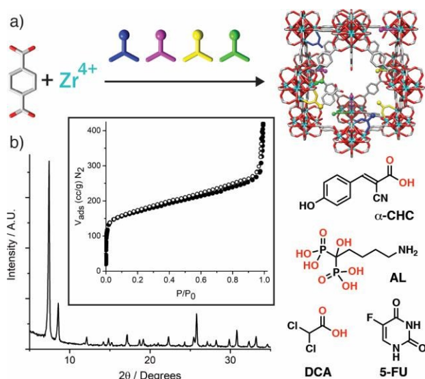
Figure 15. a) Schematic of the multivariate modulation protocol. b) Retention of crystallinity and porosity (inset) of UiO-66 when defect-loaded by multivariate modulation with three different drug molecules, \alpha -CHC, Al, and DCA, allowing postsynthetic loading of a fourth, 5-FU. Reprinted (adapted) with permission from reference 90. Copyright (2020) John Wiley & Sons.
