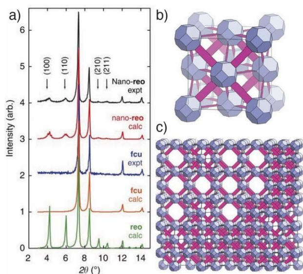
Figure 10. a) Stacked powder X-ray diffractograms of UiO-66(Hf) samples showing appearance of the reo phase in formic acid modulated syntheses (top) compared to calculated patterns for the fcu , reo , and nano- reo (nano domains of reo within fcu ) phases. b) Image of the non-defective, 12-connected fcu net of UiO-66(Hf). c) Image of missing cluster defects leading to the formation of reo nanodomains in UiO-66(Hf). Reprinted (adapted) with permission from reference 64. Copyright (2014) Springer Nature.
