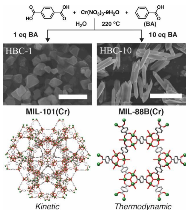
Figure 17. Schematic of benzoic acid (BA) modulated hydrothermal syntheses of Cr(III) MOFs linked by bdc, showing selection of the thermodynamic MIL-88B(Cr) phase (right, hexagonal rods, scale bar 3 \mu\text{m} ) over the kinetic MIL-101(Cr) phase (left, octahedra, scale bar 500 nm) as the modulator content in syntheses increases. Reproduced (adapted) with permission from reference 98. Published (2019) by The Royal Society of Chemistry.
