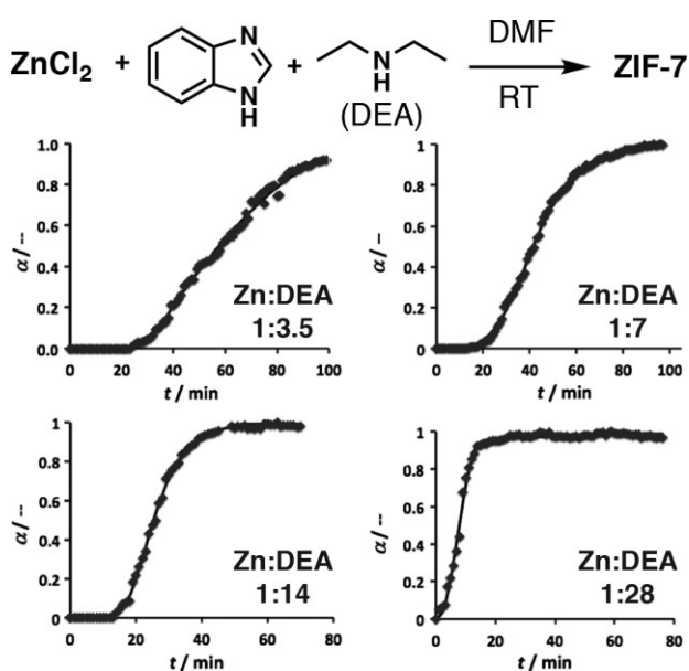
Figure 5. Experimental (symbols) and calculated (line) profiles of the evolution of the Bragg peak at Q = 5.1 \text{ nm}^{-1} from in situ wide-angle X-ray scattering data during the diethylamine (DEA) modulated self-assembly of ZIF-7, showing an increase in crystallization rate with addition of more base. Reprinted (adapted) with permission from reference 34. Copyright (2013) John Wiley & Sons.
