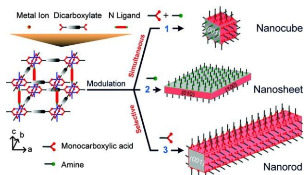
Figure 2. Schematic of face-selective coordination modulation of [\text{Cu}_2(\text{1,4-ndc})_2(\text{dabco})]_n . Reprinted with permission from reference 12. Copyright (2012) American Chemical Society.
