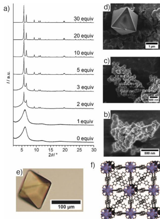
Figure 3. a) Stacked powder X-ray diffractograms of UiO-67 samples showing enhancement of crystallinity with addition of benzoic acid modulator to syntheses. Accompanying SEM images of samples modulated by b) 0 equivalents, c) 3 equivalents, and d) 30 equivalents of benzoic acid. e) A single crystal of UiO-68-NH 2 , prepared through benzoic acid modulation. f) Packing image from the crystal structure of UiO-68-NH 2 . Reprinted (adapted) with permission from reference 16. Copyright (2011) John Wiley & Sons.
