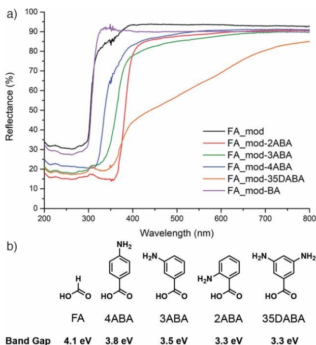
Figure 14. a) Diffuse reflectance UV/Vis spectra of formic acid modulated UiO-66 samples before (FA_mod) and after exchange of formate defects with b) different aminobenzoic acids, and the resultant experimental band gaps. Reproduced (adapted) with permission from reference 85. Published (2019) by The Royal Society of Chemistry.
