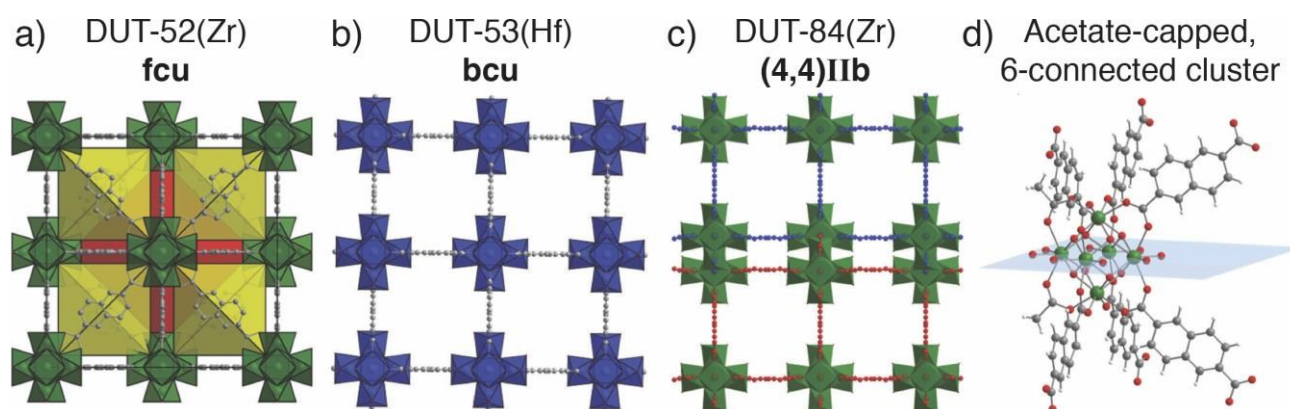
Figure 11. Crystal structure images of the MOFs formed by 2,6-ndc and Zr/Hf under acetic acid modulation. a) DUT-52 (Zr); 12-connected fcu net. b) DUT-53(Hf); 8-connected bcu net. c) DUT-84(Zr); 6-connected (4,4)IIb net. d) The ordered, acetate capped cluster of DUT-84(Zr). Reproduced (adapted) with permission from reference 66. Published (2013) by The Royal Society of Chemistry.
