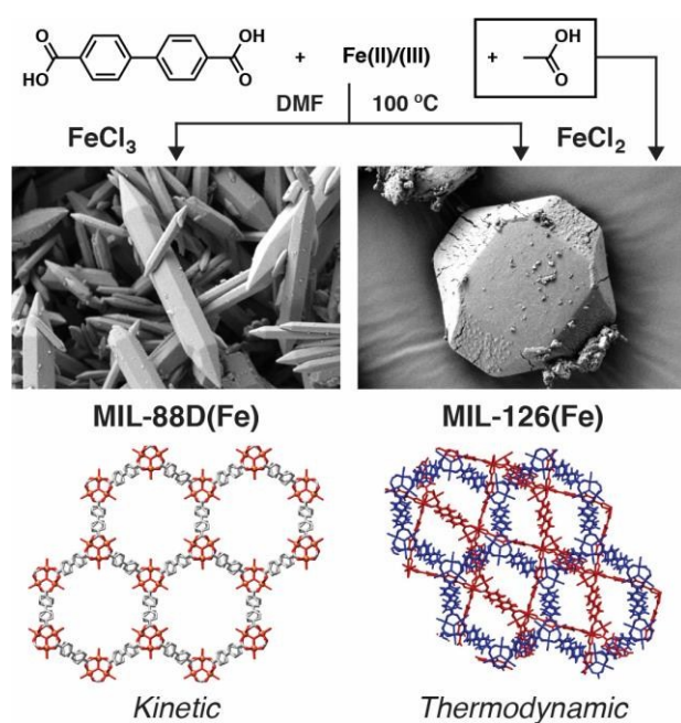
Figure 19. Schematic of the oxidation modulation protocol to select between kinetic and thermodynamic phases in the self-assembly of Fe-bpdc MOFs, which mirrors the control offered by coordination modulation. Reprinted (adapted) with permission from reference 77. Copyright (2019) American Chemical Society.
