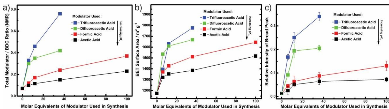
Figure 12. Close alignment of different properties of samples of UiO-66 modulated with differing carboxylic acids. a) Total modulator incorporation from ^1\text{H} NMR spectra of digested samples. b) BET surface areas from \text{N}_2 adsorption/desorption isotherms. c) Presence of the reo defect phase from intensity of peaks in powder X-ray diffractograms. Reprinted with permission from reference 70. Copyright (2016) American Chemical Society.
