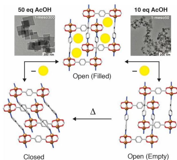
Figure 8. Schematic of size-induced shape memory in [Cu 2 (1,4-bdc) 2 (4,4'-bipy)] n which occurs for 50 nm particles (right) but not >300 nm particles (left). Reprinted in part (adapted) with permission from reference 53. Copyright (2013) The American Association for the Advancement of Science.
