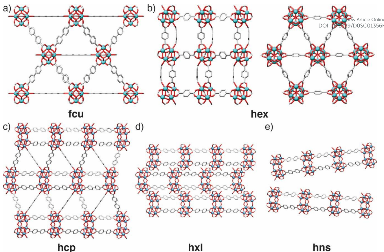
Figure 18. Solid-state structures of different topologies accessible within the phase space of Zr MOFs linked by linear dicarboxylate ligands. a) UiO-67 in the fcu topology. b) The Zr-bdc MOF which is a polymorph of UiO-66 but has hex topology, viewed down the b (left) and c (right) crystallographic axes. c) The hcp phase formed by Hf and bpdc. d) The hxl phase formed by Hf and bpdc, which can spontaneously arise from the hcp phase by loss of bpdc. e) The hns phase of Hf and bpdc, which is a delaminated version of the hxl phase.
