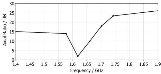
Figure 7. Axial Ratio vs Frequency (Theta = 0, Phi = 0).
