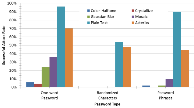
Figure 5: Successful attack rates are lowest against passwords masked with Color-halfTone and Crystallize filters. Gaussian-Blur and Mosaic filters perform well with random characters and passphrases. Guesses against Plain text are the most successful, followed by Asterisks because of revealing the entered character briefly before masking it.
