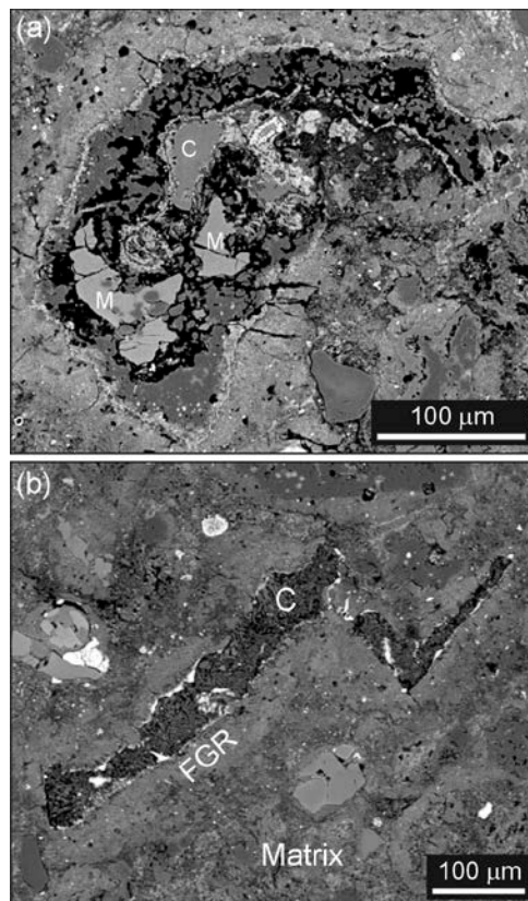
Fig. 1. Backscattered electron SEM images. (a) A CAI containing melilite (M) and calcite (C). (b) An object with an unusually high aspect ratio that is almost entirely composed of finely crystalline calcite. This object has a fine-grained rim (FGR).
