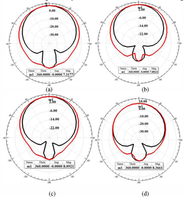
Fig. 6 Directivity Plot (a) Single rectangular antenna (b) Double rectangular antenna (c) Double circular antenna (d) Rectangular-circular antenna
