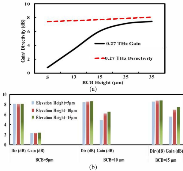
Fig. 4 (a) Plot of BCB height change vs gain/directivity (b) Plot of Stack height with fixed BCB height
