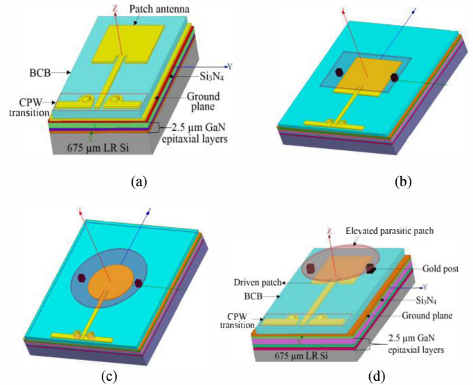
Fig. 1 Schematic of microstrip patch antenna (a) Single-rectangular [15] (b) Double-rectangular (c) Double-Circular (d) Rectangular-circular antenna [16]
