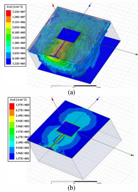
Fig. 2 Electromagnetic Simulation of volume current in the entire circuit design (a) when the substrate is not shielded (b) when the substrate is shielded
