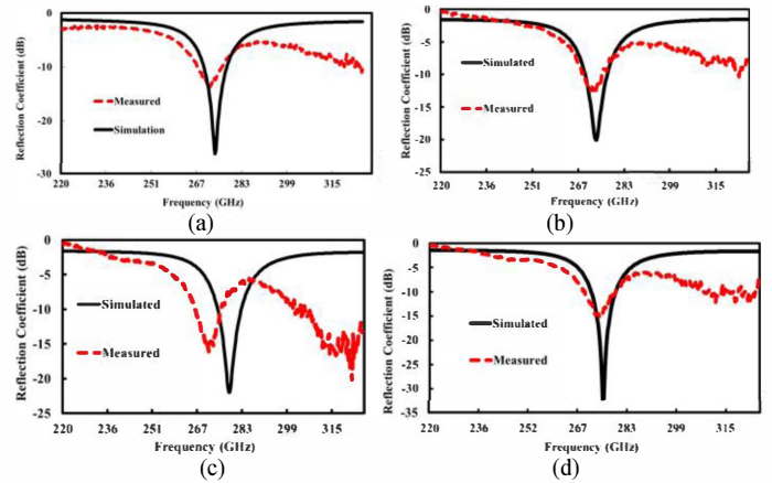
Fig. 5 Reflection Co-Efficient Plot (a) Single rectangular antenna (b) Double rectangular antenna (c) Double circular antenna (d) Rectangular-circular antenna
