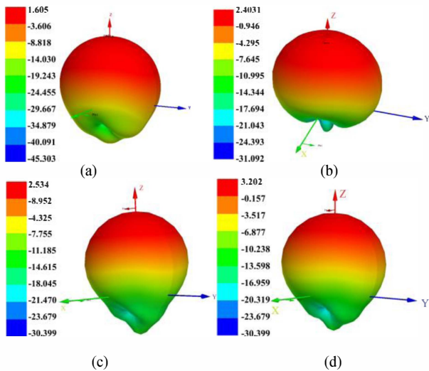
Fig. 7 Gain Plot (a) Single rectangular antenna (b) Double rectangular antenna (c) Double circular antenna (d) Rectangular-circular antenna
