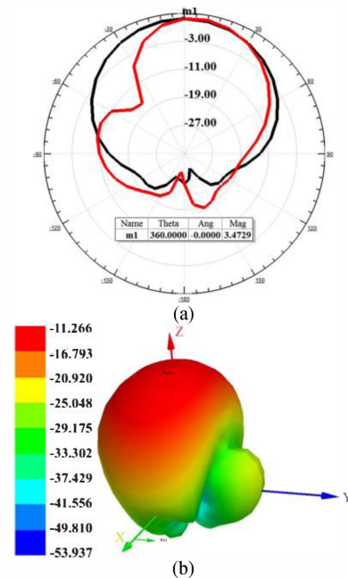
Fig. 3 BCB as stack substrate (a) Directivity (b) Gain
