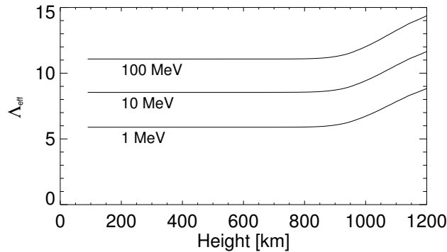
Figure 7. The effective Coulomb logarithm, \Lambda_{eff} through the atmosphere for protons of energy 1, 10 and 100 MeV.
