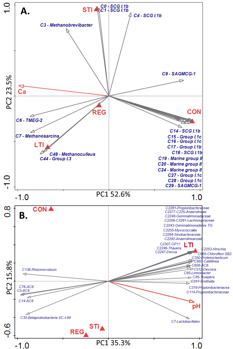
Fig 1. Db-RDA and two dimensional ordination plots of (A) archaeal communities and (B) bacterial communities of studied soils based on Bray-Curtis distance matrix. In (A), ordinations show the 20 best fitting archaeal OTUs are plotted together with centroids of soil samples. In (B), ordinations of the 30 best fitting bacterial OTUs are shown. Significant explanatory variables are indicated by the red arrows. The percentage of community distribution explained by each axis is indicated in the figures. (TIF)
