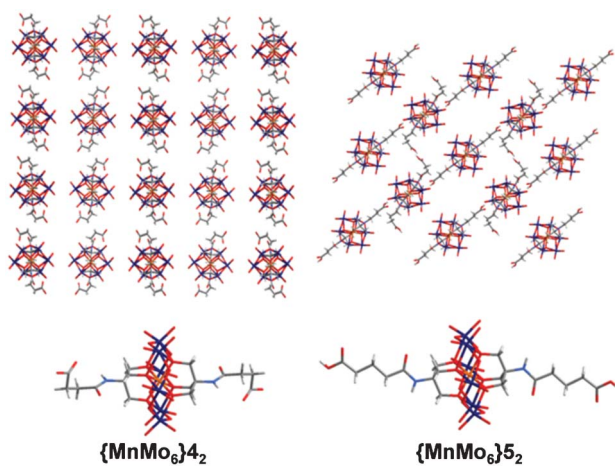
Fig. 3 X-Ray Structures of \{MnMo_6\}_{4_2} (top and bottom left, the structure is disordered) and \{MnMo_6\}_{5_2} (top and bottom right). The packing diagram for \{MnMo_6\}_{4_2} is shown in the (xy) plan and for \{MnMo_6\}_{5_2} in the (yz) plan. The TBA cations and the solvent molecules are removed from the packing diagrams for clarity. Colour scheme: O (red), Mo (dark blue), Mn (orange), N (light blue), C (dark grey) and H (light grey).
