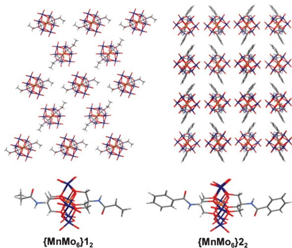
Fig. 2 X-Ray structures of \{MnMo_6\}_{12} (top and bottom left) and \{MnMo_6\}_{22} (top and bottom right). The two packing diagrams are shown in the (yz) plan. Colour scheme: O (red), Mo (dark blue), Mn (orange), N (light blue), C (dark grey) and H (light grey). The TBA cations and the solvent molecules are removed from the packing diagrams for clarity.
