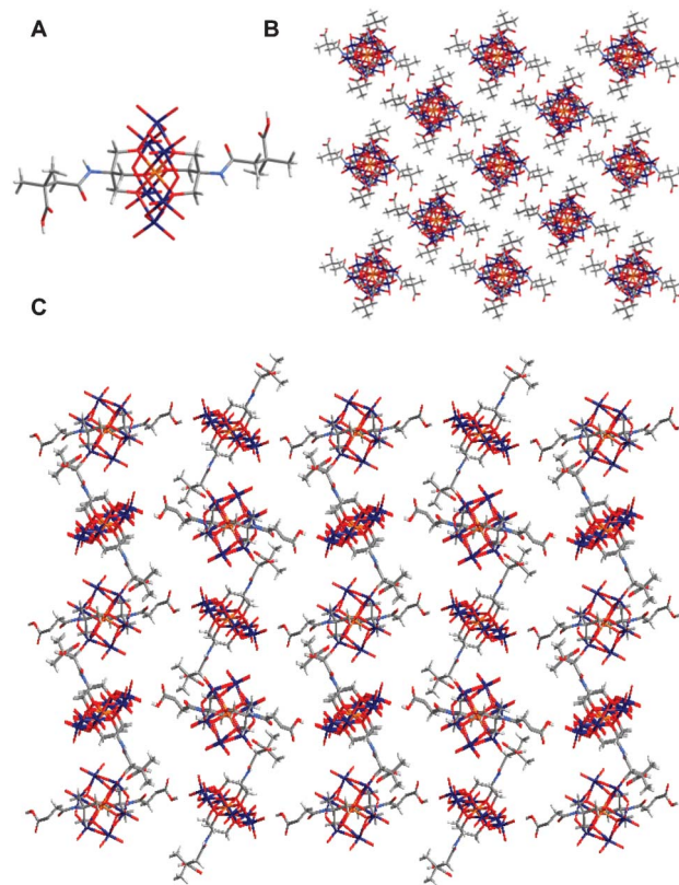
Fig. 4 A) Crystal structure of (a)- \{MnMo_6\}_{6_2} ; B) Packing diagram of (a)- \{MnMo_6\}_{6_2} in the (xz) plan and C) evidence of the H-bonding network in the (yz) plan. Colour scheme: O (red), Mo (dark blue), Mn (orange), N (light blue), C (dark grey) and H (light grey). The TBA cations and the solvent molecules are removed from the packing diagrams for clarity.
