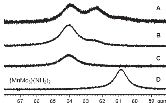
Fig. 1 1 H NMR spectra in d 6 -DMSO of \{MnMo_6\}_6 synthesised in different conditions. (C_2O_3)_6 is reacted with \{MnMo_6\}(NH_2)_2 following the conditions described in Table 1: A) 10 equivalent in MeCN, B) 10 equivalents in DMF, C) 20 equivalents in DMF and D) NMR of the hybrid precursor \{MnMo_6\}(NH_2)_2 in d 6 -DMSO.
