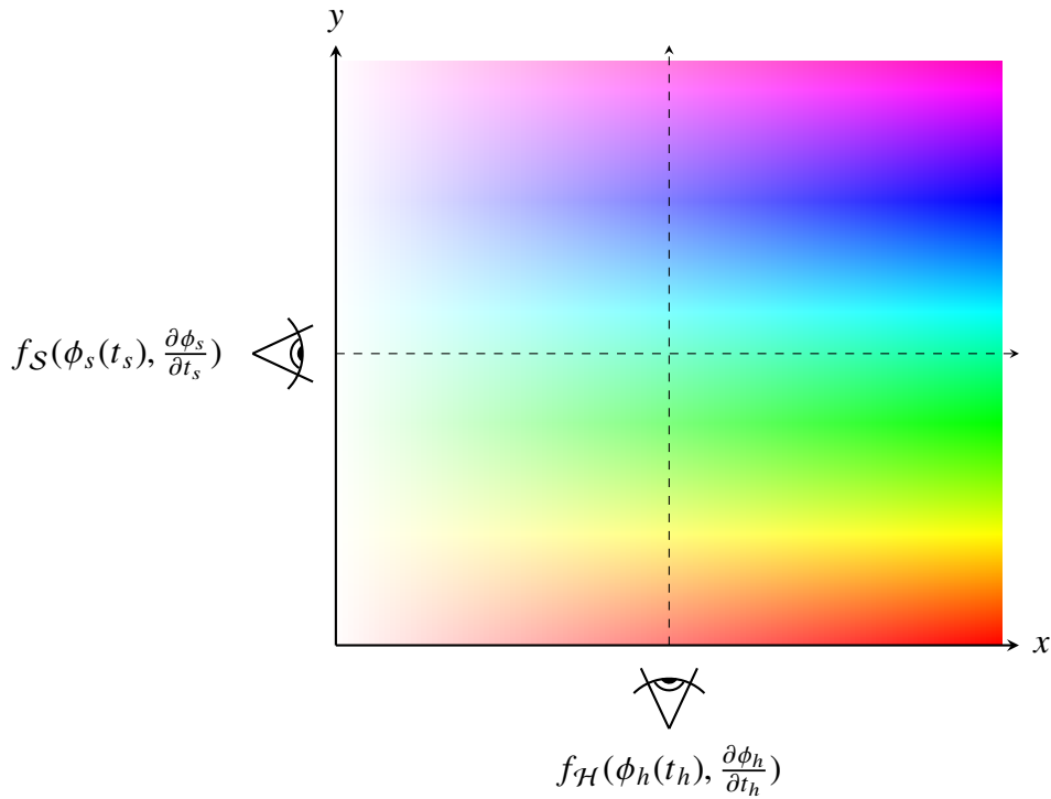
Figure 3: Two continuously varying quantities that can be used to develop differential equations from two different perspectives.
