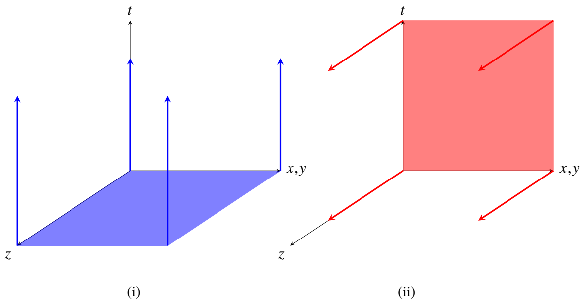
Figure 1: A representation of temporal and spatial evolution: (i) represents an extrapolation through time via the laws; (ii) represents the analogous extrapolation through space.
