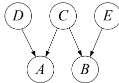
Fig. 1: A common cause structure that gives rise to spurious regularities.
