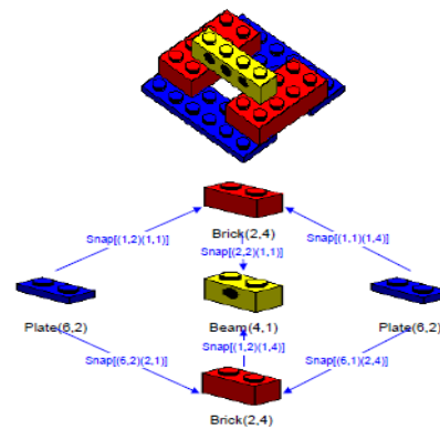
Figure 5. An example of a LEGO assembly structure and a corresponding assembly graph [Pey03]
