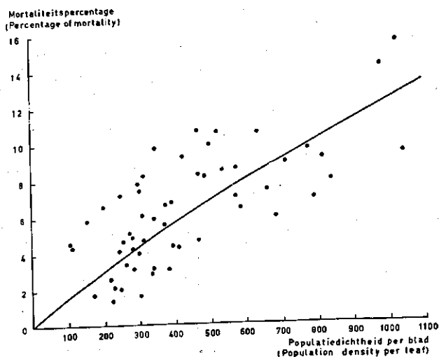
FIG. 54. Relationship between population density and natural mortality of T. urticae .
