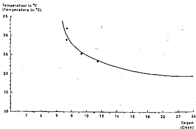
FIG. 5. Relationship between the temperature and the time required for development of S. punctillum from hatching to adult
