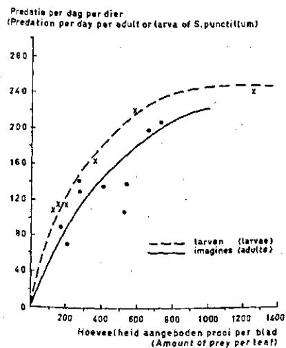
FIG. 56. Relationship between the population density of T. urticae and the predation by S. punctillum (20-25°C)
