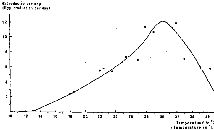
FIG. 3. Relationship between the temperature and the egg production of T. urticae per day
