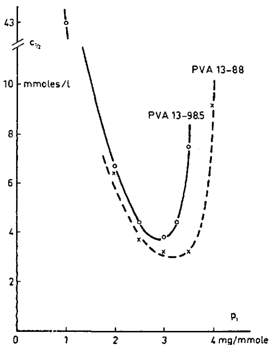
FIG. 5-10. Dependence of the critical salt concentration on the polymer dosage. sol C; \varphi_1 = 0.5 ; c_{sol} = 3 mmoles/l; t_1 = 15 min; t_2 = 1 h.
