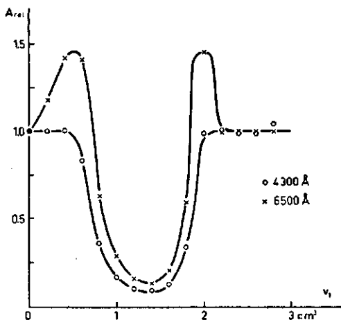
FIG. 5-2. The flocculation of AgI sol with PVA as measured by the relative absorbance. Sol A, PVA 3-98.5; p_1 = 2.5 \text{ mg PVA/mmmole AgI} ; c_{sol} = 3 \text{ mmoles/l} ; c_s = 10 \text{ mmoles KNO}_3/\text{l} ; t_1 = 15 \text{ min} ; t_2 = 1 \text{ h} .
