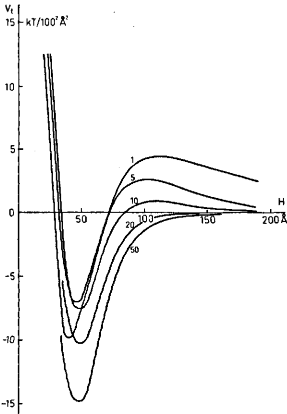
FIG. 6-10. The total free energy of interaction between a covered and an uncovered particle in the presence of several concentrations of \text{KNO}_3 (mmoles/l). \psi_d = -90 \text{ mV} , p_s = 0.9 \text{ mg/m}^2 , A'_0 = 0.010 \text{ \AA}^{-2} , \epsilon_s = 1 kT and l_s = 16.9 \text{ \AA} .
