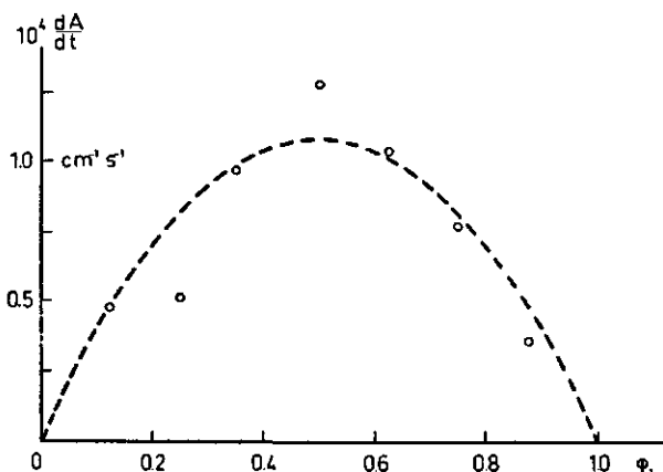
FIG. 5-15. The initial rate of flocculation as a function of \varphi_1 (two portion method). The broken line corresponds to dA/dt = 4.3 \cdot 10^{-4} \varphi_1 \varphi_2 \text{cm}^{-1} \text{s}^{-1} . PVA 13-98.5, sol C; c_{\text{sol}} = 0.2 mmole/l; c_s = 15 mmoles \text{KNO}_3 /l; p_1 = 2.5 mg PVA/mmole of AgI.
