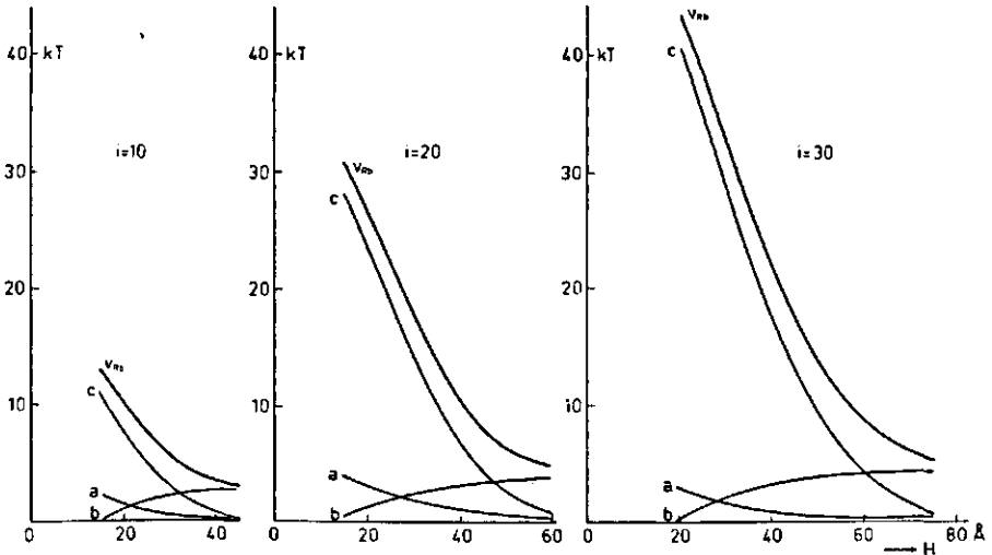
FIG. 6-6. The configurational repulsion free energy v_{Rb} and its components (a, b and c) as a function of the interparticle distance for one single loop of 10, 20 or 30 statistical chain element elements, respectively, calculated according to eq. (6-16).
