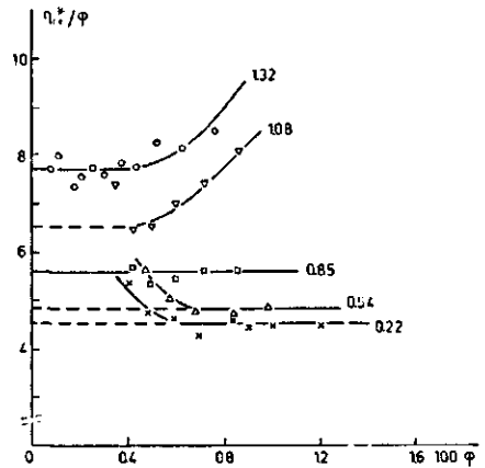
FIG. 4-3. The reduced viscosity ratio excess of silver iodide (sol C), covered with PVA 60-99, as a function of the volume fraction of AgI. The figures at the right indicate the amount of PVA adsorbed (mg/m 2 ).
