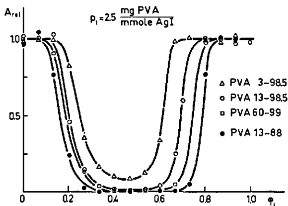
FIG. 5-5. The flocculation as a function of the ratio of the amounts of covered and uncovered sol at a constant polymer dosage of 2.5 mg PVA/mmole AgI of the first portion. c_{sol} = 3 mmoles/l; c_2 = 10 mmoles KNO_3 /l; t_1 = 15 min; t_2 = 1 h. The curve for PVA 13-88 has been measured with sol B, the others with sol A.
