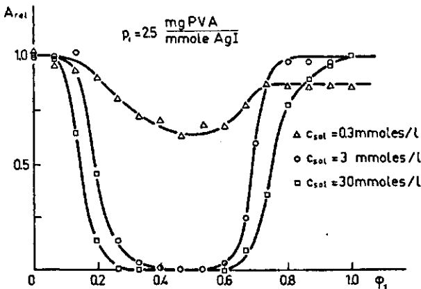
FIG. 5-11. The flocculation of AgI (sol A) by PVA 13-98.5 at different sol concentrations. p_1 = 2.5 mg PVA/mmole AgI; c_e = 10 mmoles \text{KNO}_3/\text{l} ; t_1 = 15 min; t_2 = 1 h.
