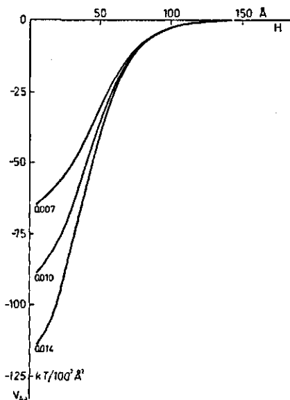
FIG. 6-3. The adsorption attraction free energy as a function of the interparticle distance for p_a = 0.9 \text{ mg PVA/m}^2 . The value for the coverage in the first layer on the second particle ( A'_0 in \text{\AA}^{-2} ) is given for each curve. The adsorption free energy per segment, \epsilon_a , was taken to be 1 kT .
