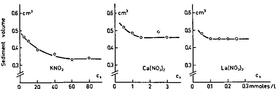
FIG. 5-17. The sediment volume after 200 h of standing of 0.30 mmole AgI (sol C) flocculated with PVA 13-98.5 as a function of the salt concentration. p_1 = 2.5 mg PVA/mmol AgI; \phi_1 = 0.5 ; t_1 = 15 min.
