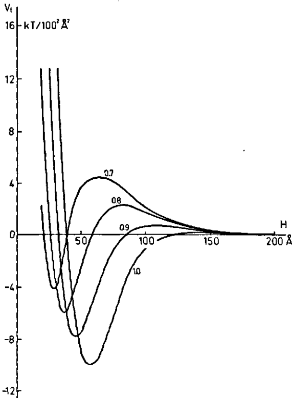
FIG. 6-13. The total interaction free energy at several amounts of adsorbed polymer ( p_a in \text{mg/m}^2 ). \text{KNO}_3 , c_s = 10 mmoles/l, \psi_d = -90 mV; A'_0 = 0.010 \text{ \AA}^{-2} , \epsilon_s = 1 kT and l_s = 16.9 \text{ \AA} .
