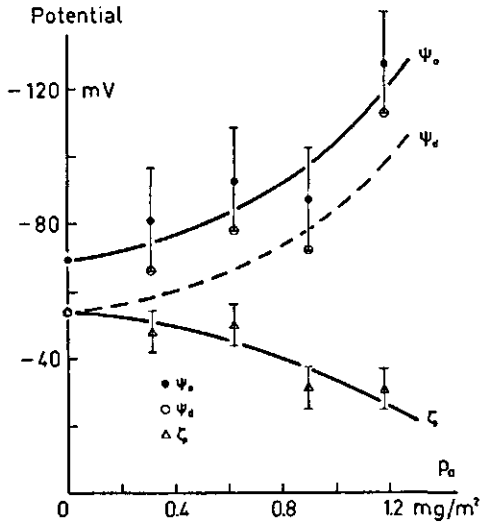
FIG. 4-5. Electrophoretic measurements on AgI (sol C) covered by PVA 16-98. The \zeta -potential, surface potential ( \psi_0 ) and STERN potential ( \psi_d ) at the beginning of the mobility plateau as a function of p_a .
