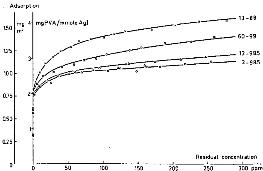
FIG. 3-2. The adsorption of polyvinyl alcohol on silver iodide (sol C); sol concentration 50 mmoles/l; time of adsorption 1 hour
