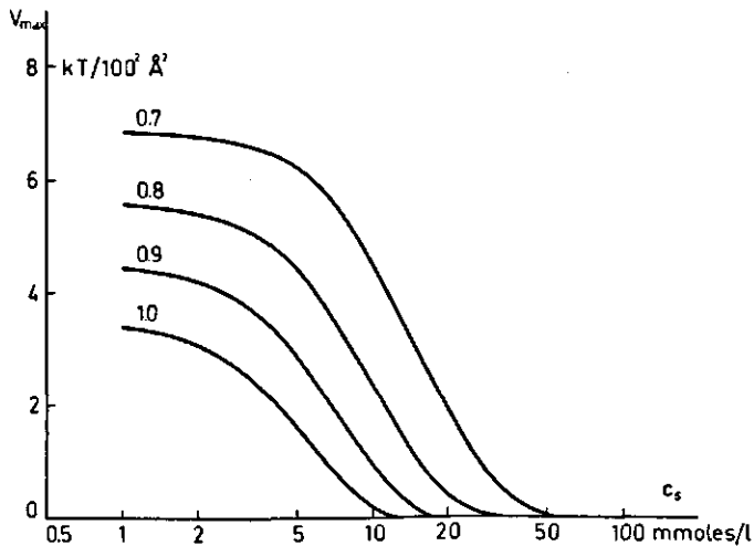
FIG. 6-14. The height of the maximum in the free energy of interaction curve as a function of the concentration of \text{KNO}_3 ( \psi_d = -90 \text{ mV} ) at several amounts adsorbed ( p_a in \text{mg/m}^2 ).
