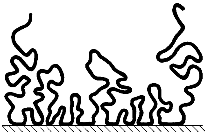
FIG. 4-9. Schematic representation of an adsorbed polymer layer at high coverage. The middle section of an adsorbed molecule assumes a distribution of loops according to HOÈVE; beyond the first layer the segment density distribution is exponential. At the ends of a molecule tails can be present.
