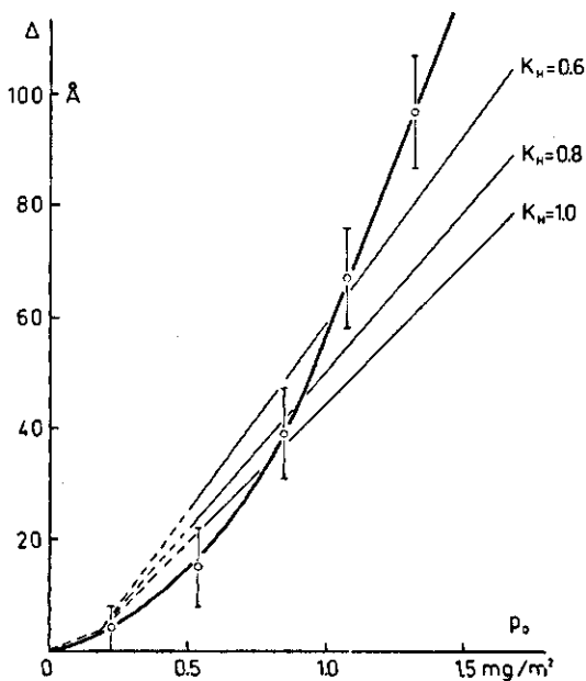
FIG. 4-8. The theoretical thickness calculated from eq. (4-29), compared with the experimental thickness measured by viscosimetry. The theoretical lines were calculated using 10^4 \rho_0 = 70 \text{ \AA}^{-3} and 10^4 \rho_{eff} = 5 \text{ \AA}^{-3} .
