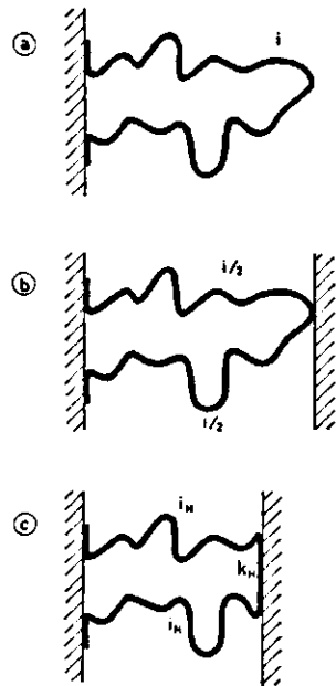
FIG. 6-5. Schematic representation of the bridging process. a. At large interparticle distances a loop of i elements has its undisturbed configuration b. After adsorption of the first element two bridges of i/2 elements each are formed c. At shorter distances two bridges of i_H elements are present and a train of k_H elements has been adsorbed on the second surface.
