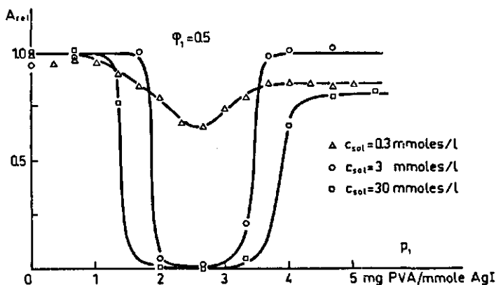
FIG. 5-12. The flocculation of AgI by PVA 13-98.5 at different sol concentrations. \varphi_1 = 0.5 ; c_s = 10 mmol KNO 3 /l; t_1 = 15 min; t_2 = 1 h. The curve for c_s = 3 mmol/l was measured with sol C, the others with sol A.
