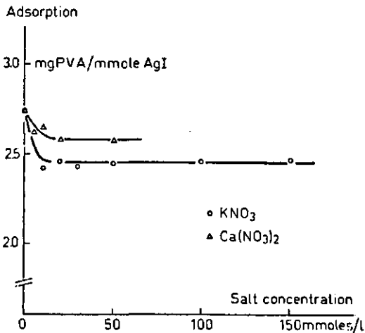
FIG. 3-3. Effect of the salt concentration on the adsorption of PVA 13-98.5 on AgI (sol C) sol concentration 50 mmoles/l; polymer concentration (added) 240 ppm
