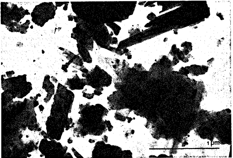
Fig. 14. Electron micrograph of the clay fraction of sample 62 (TFDL).
