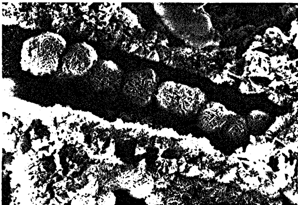
Fig. 15. Scanning electron micrograph of silicified chalk from the Platte Bos (TFDL). Magnification 2000 \times .
