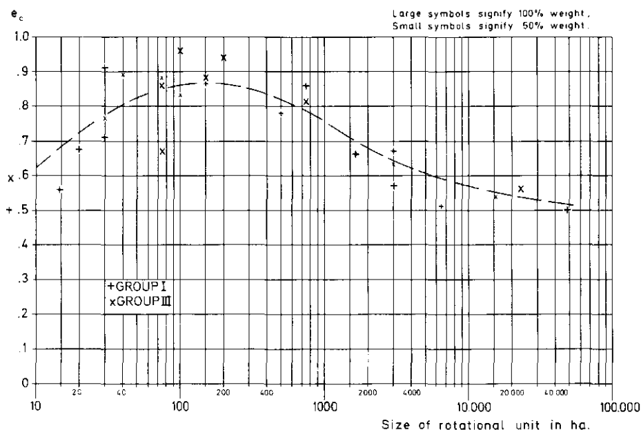
Fig.6. Influence of size rotational unit on conveyance efficiency (surface irrigation).
