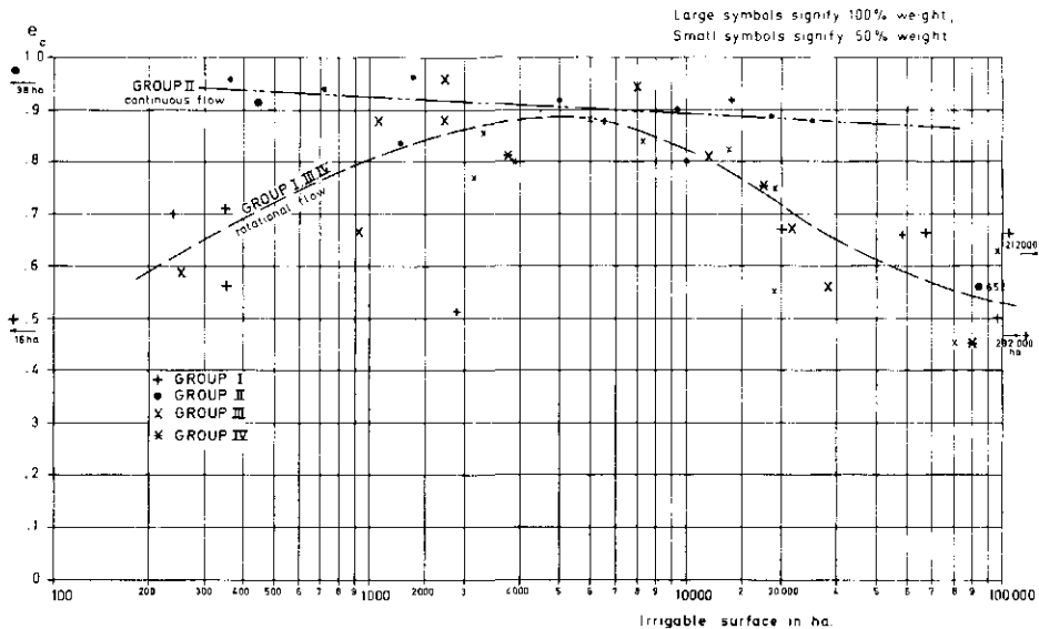
Fig.5. The e_c -values as a function of the irrigable area.
