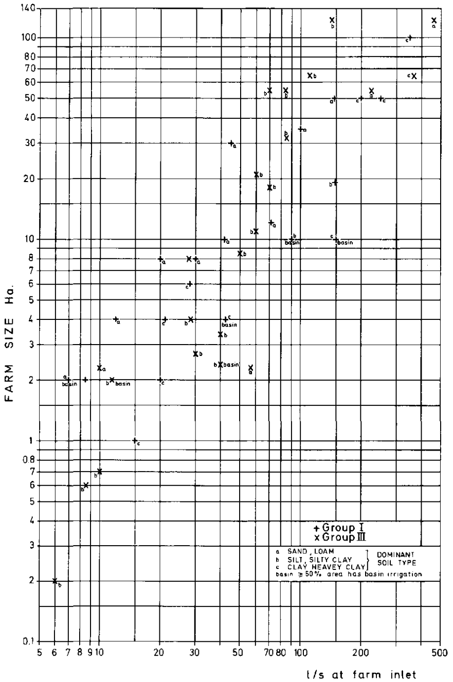
Fig. 8. Relation of farm size to discharge at farm inlet.
