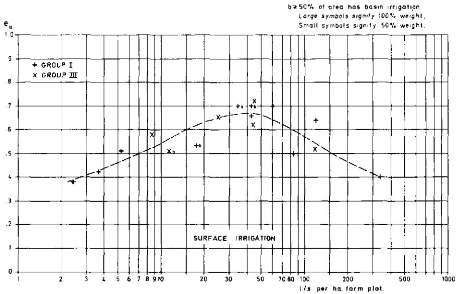
Fig.14. Influence of flow rate per ha farm plot on e_a .
