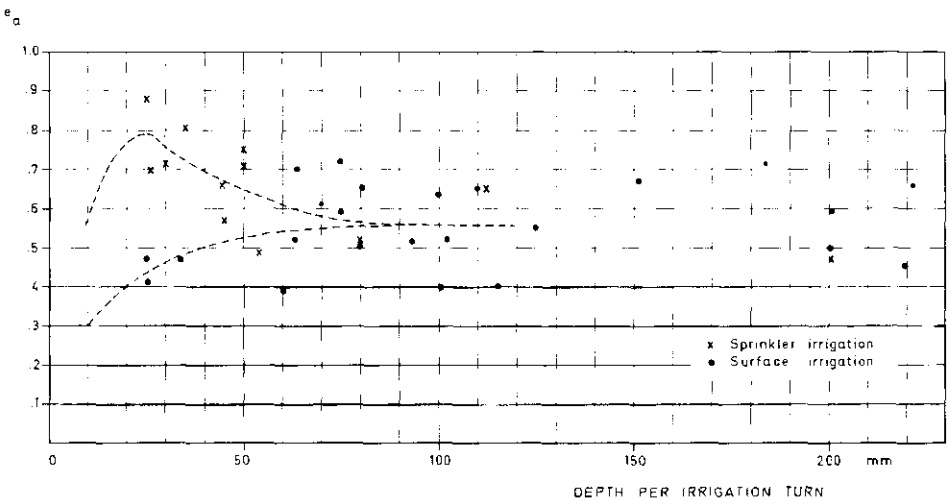
Fig.12. Relation of field application efficiency to depth of application per irrigation.
