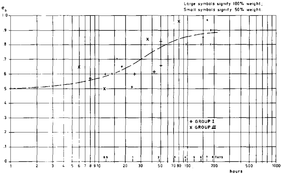
Fig.9. Influence of average delivery period at farm inlet on farm ditch efficiency (surface irrigation).
