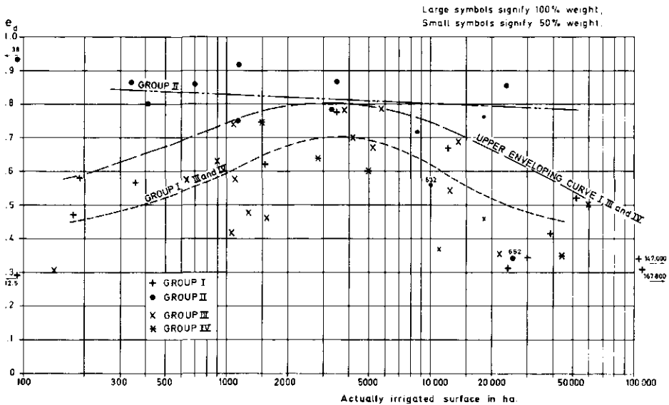
Fig.17. Relation of distribution efficiency to average total area which is irrigated at least once per year.
