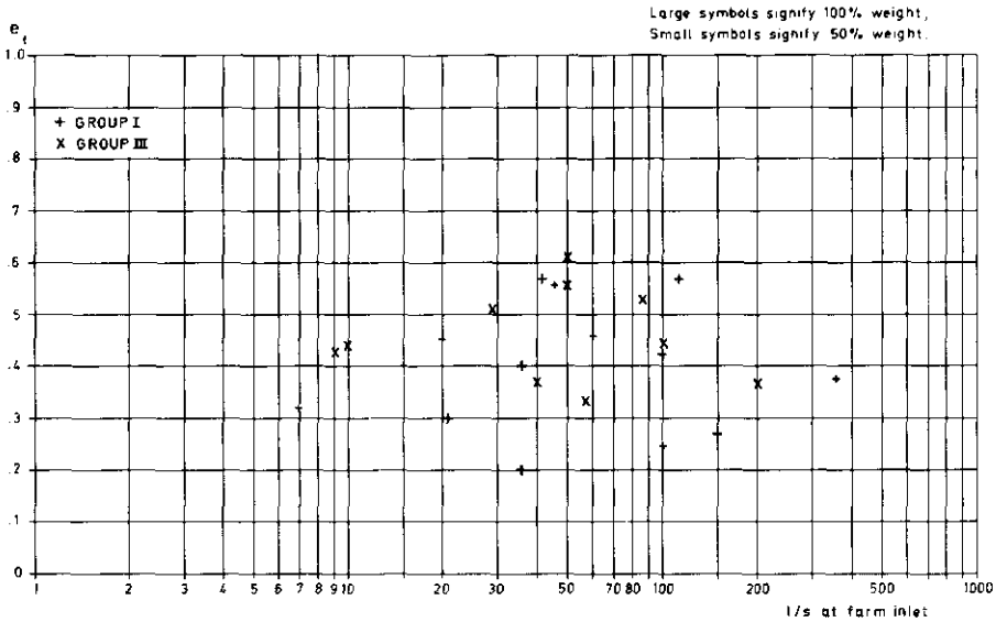
Fig.15. Influence of flow rate at farm inlet on e_f .
