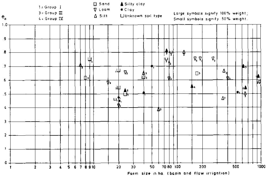
Fig.13. Relation of field application efficiency with farm size and dominant soil type.
