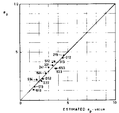
Fig.19. Correlation of estimated and calculated efficiency values.
