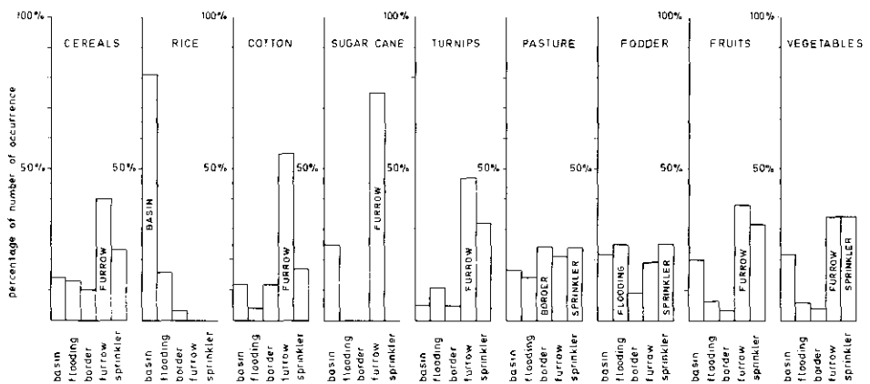
Fig.2. Field irrigation method as a function of irrigated crops (see Tab.2).
