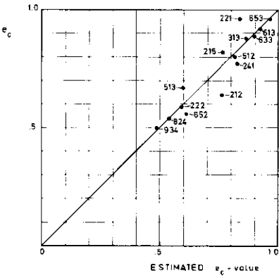
Fig.19. Correlation of estimated and calculated efficiency values.
