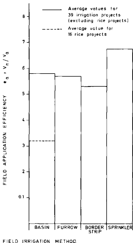
Fig.10. Field application efficiency related to irrigation methods.
