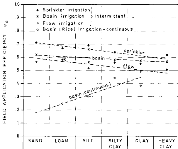
Fig.11. Field application efficiency and method with reference to soil type.
