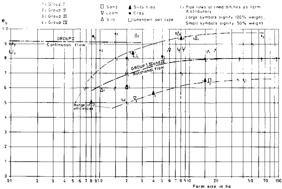
Fig.7. The e_b as a function of farm size and dominant soil type.
