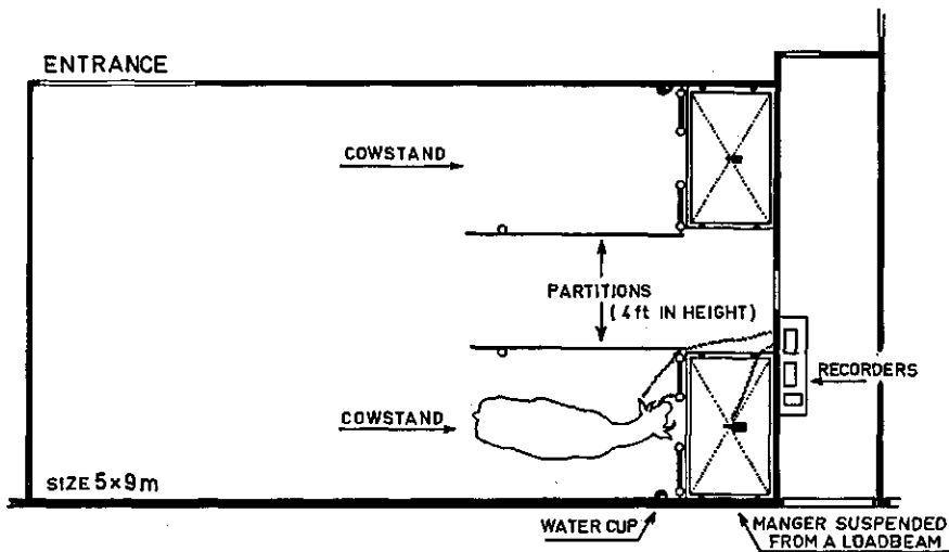
FIG. 2.1. Plan of the experimental room.
