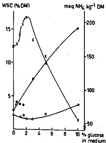
Fig. 25. Water-soluble carbohydrate content of roots after 4h of incubation in glucose solutions of different concentration (●) and after 4h of subsequent NH 4 -uptake (○). NH 4 uptake (x) indicated on the right-hand ordinate. Experiment 23.
