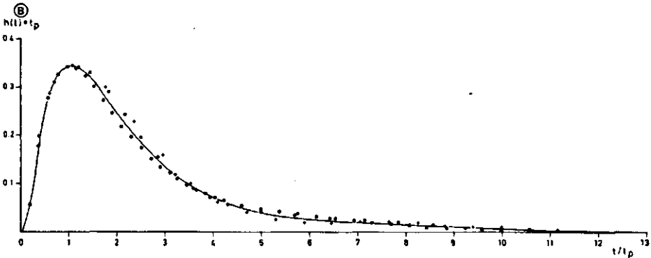
Fig. A3.5. Basic shape of IUH. A. Duration T=16 . B. Duration T=3 . \bullet\bullet\bullet from p=1 , \circ\circ\circ from p=4 , +++ from p=16 .
