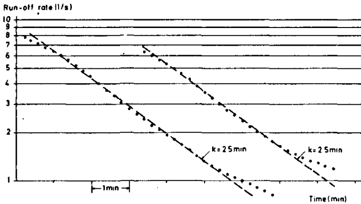
Fig. 3. Recession curves from experiments at De Nieuwlanden. k is parameter of the linear reservoir model.
