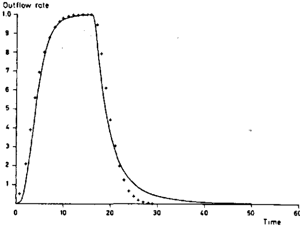
Fig. A3.3. Linear reconstruction of outflow for T 16. — calculated outflow, ++ reconstructed outflow.
