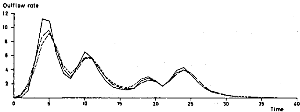
Fig. A3.13. Quasilinear simulation of outflow with the peak of outflow, q_p , as criterion, using the basic shape of IUH ( T=3 ). — calculated outflow, - - - linear simulation, - · - quasilinear simulation. Sum of squared differences: linear simulation 20.8, quasilinear simulation 11.8.
