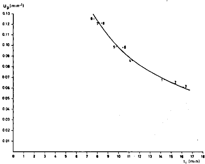
Fig. 33. Relation between the peak of the IUH, U_p , and the lag time of IUH, t_l .
