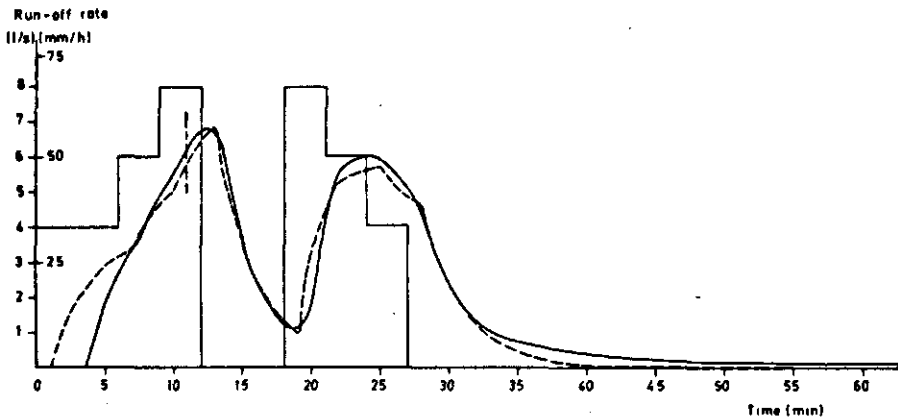
Fig. 4. Run-off simulation with the lag-and route model. The parameters were optimized for this storm according the least sum of squared differences (LS). Data from De Nieuwlanden experiments. \square rainfall, — observed run-off, --- simulated run-off. Parameters: k = 3.1 min, \tau = 1.0 min. LS: 8.22 \text{ l}^2/\text{s}^2 ( t = 11-63 min).
