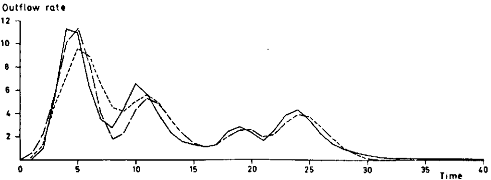
Fig. A3.9. Quasilinear simulation of outflow with the peak of outflow, q_p , as criterion for choosing one IUH out of three ( T = 16 ). — calculated outflow, - - - linear simulation, - · - quasilinear simulation. Sum of squared differences: linear simulation 47.7, quasilinear simulation 22.2.
