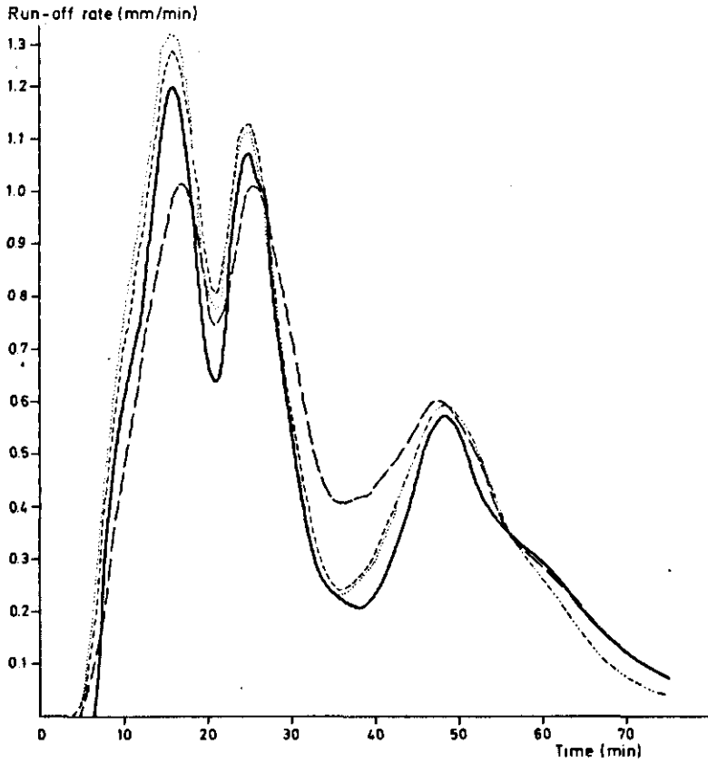
Fig. 28. Linear and quasilinear simulations of run-off for Event A23. ▨ losses, — observed run-off, --- linear simulation, ..... quasilinear simulation (first time), - · - · - quasilinear simulation (second time). Sum of squared differences: linear simulation 0.87 \text{ mm}^2/\text{min}^2 , quasilinear simulation 0.46 \text{ mm}^2/\text{min}^2 .
