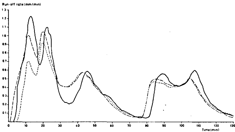
Fig. 15. Run-off simulations with the Nash cascade for Event A23 from Table 2 (Gray Haven). The model parameters were estimated by moment fitting for Storm 7 from Table 3 for the loss models initial loss + \Phi index and initial loss + proportion assumed lost, — observed run-off, - - - proportion assumed lost, ···· \Phi index.
