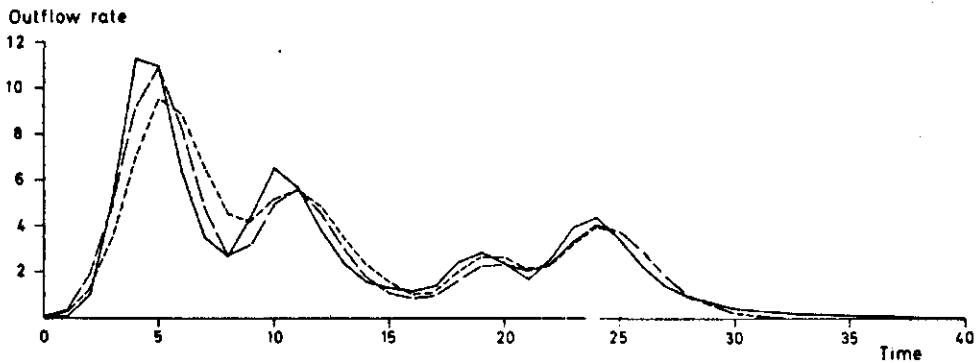
Fig. A3.11. Quasilinear simulation of outflow with the peak of outflow, q_p , as criterion, using the basic shape of IUH ( T 16 ). — calculated outflow, ---- linear simulation, - - - quasilinear simulation. Sum of squared differences: linear simulation 47.7, quasilinear simulation 19.1.
