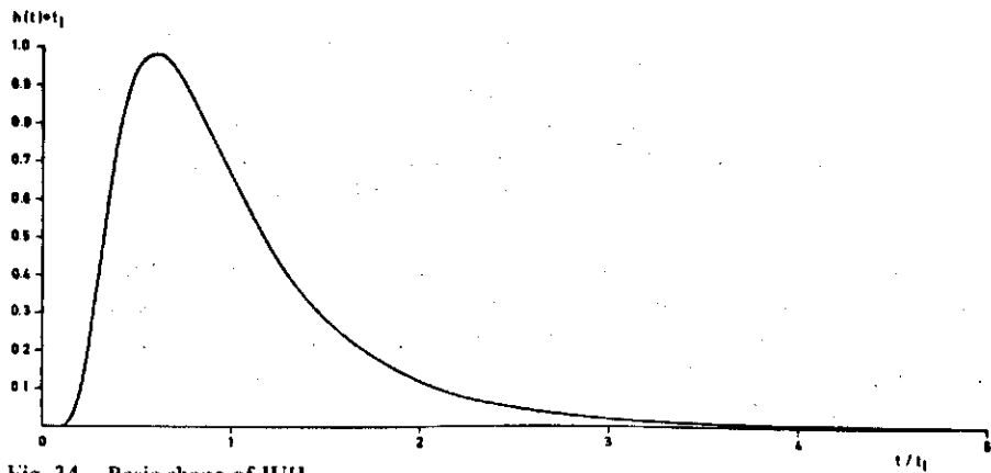
Fig. 34. Basic shape of IUH.
