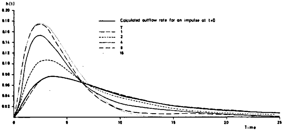
Fig. A3.1. Instantaneous unit hydrographs, h(t) , for p=1 and T variable.
