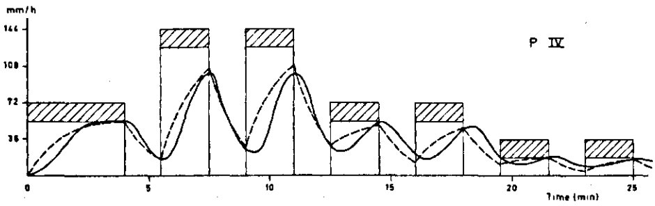
Fig. 12. Run-off simulations with the linear reservoir model. The values for the lag times were obtained from the recession curve (Fig. 11, Pomona). ▨ rainfall, ▩ infiltration, — observed run-off, --- simulated run-off. P III: k = 1 \text{ min } 26 \text{ s} , P IV: k = 1 \text{ min } 12 \text{ s} .
