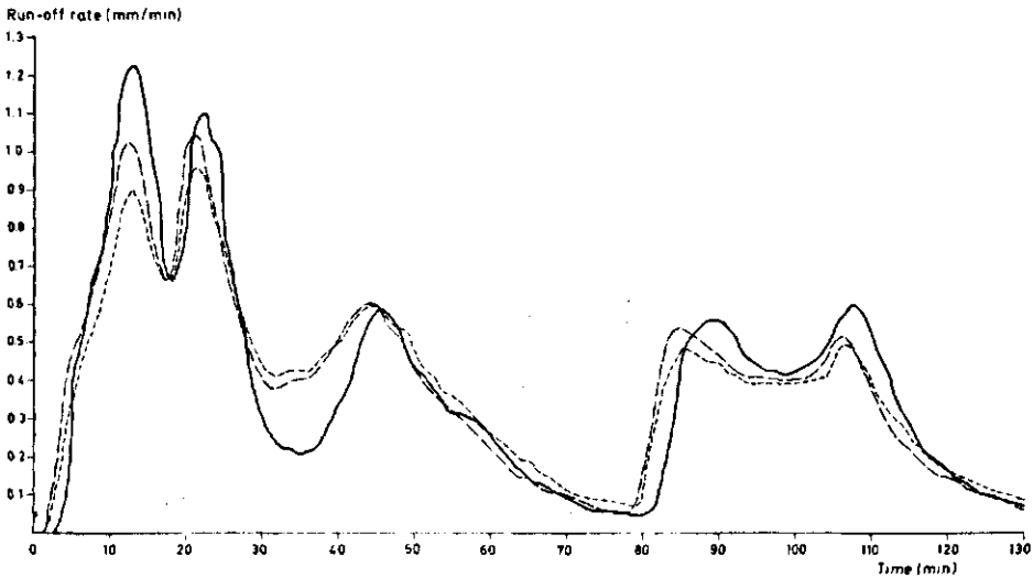
Fig. 18. Run-off simulations with the model convective diffusion, upstream inflow, for Event A23 from Table 2 (Gray Haven). The model parameters were estimated by moment fitting for Storm 8 from Table 3 for the loss models \Phi index and proportion assumed lost. — observed run-off, ---- proportion assumed lost, -.-.- \Phi index.
