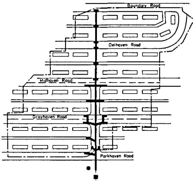
Fig. 19. Plan of the Gray Haven catchment area. --- catchment boundary, ● raingauge, ■ Parshall flume, ■■■ drainage system.
