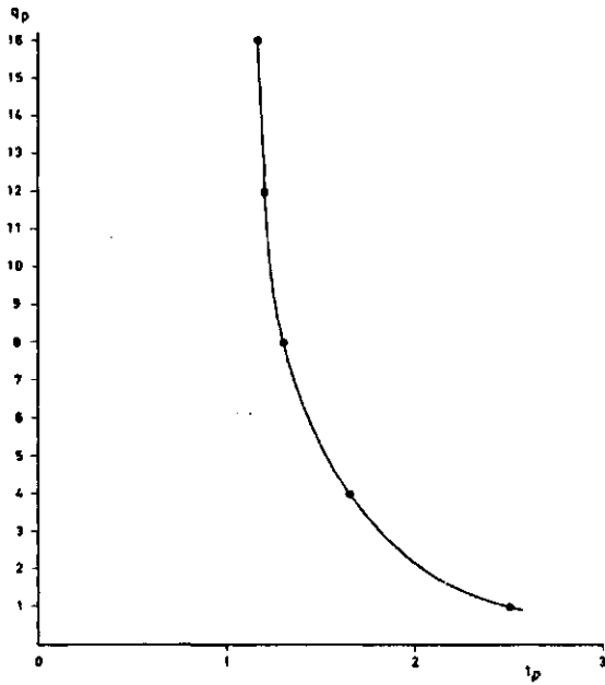
Fig. A3.10. Relation between the peak of outflow, q_p , and the time to peak of the IUH, t_p , for T 16 .
