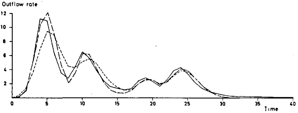
Fig. A3.8. Quasilinear simulation of outflow with the average inflow \bar{p} . Extent of influence for calculating \bar{p} is 1 time unit. — calculated outflow, - - - linear simulation, - · - quasilinear simulation.
