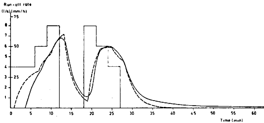
Fig. 6. Run-off simulation with the lag-and-route model. The lag time was obtained from the recession curves in Figure 3. \square rainfall, — observed run-off, --- simulated run-off. Parameters: k = 2.5 min, \tau = 1.0 min. LS: 12.91 \text{ l}^2/\text{s}^2 ( t = 11-63 min).
