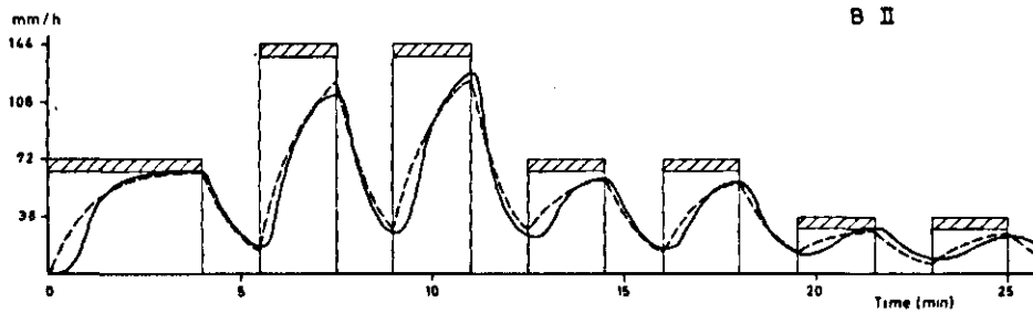
Fig. 14. Run-off simulation with the linear reservoir model. The value for the lag time was obtained from the recession curve of the Bennekom data. k = 1 min. ▨ rainfall, ▩ infiltration, — observed run-off, - - - simulated run-off.
