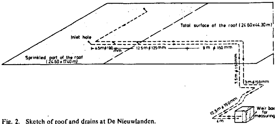
Fig. 2. Sketch of roof and drains at De Nieuwlanden.
