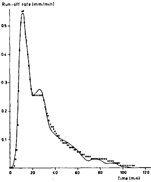
Fig. 24. Reconstruction of run-off rate for Storm 8. x observed run-off, — re-constructed run-off.
