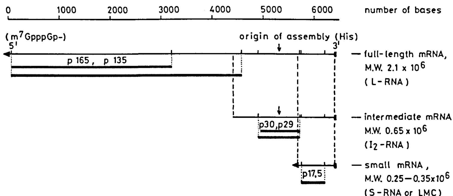
FIG. 1.1. Genetic map of TMV.
