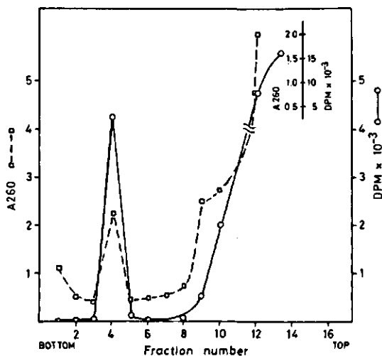
FIG. 4.4. Sedimentation profile of the 27,000 xg supernatant of TMV infected tobacco protoplasts after CsCl centrifugation.
