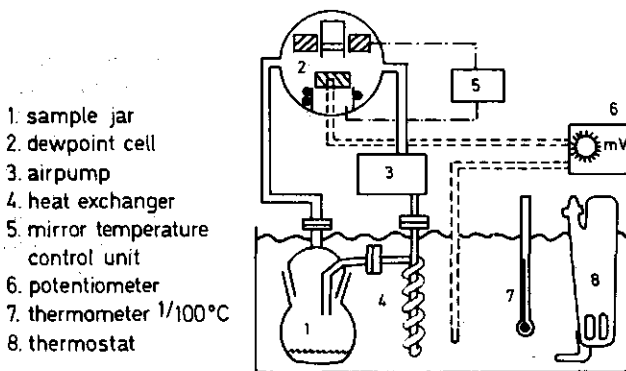
Figure 1. Scheme of the wateractivity measuring device.
