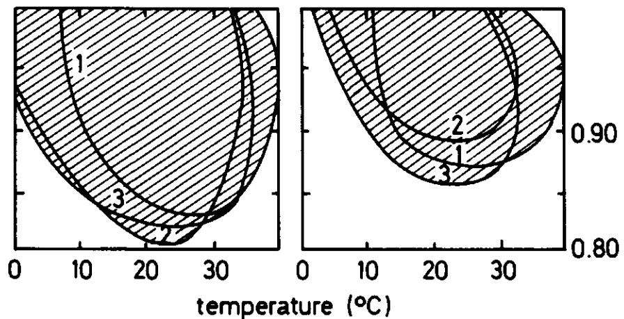
Figure 1. Conditions of water activity ( a_w ) and temperature favorable (shaded area) for mycotoxin production by different fungal species. Data are obtained with different fungal strains and substrates.
