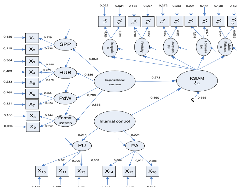
Gambar 1. SEM-PLS
