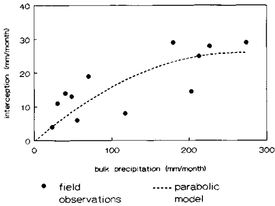
Fig. III.4 Comparison of parabolic interception model without zero degree term and observed (Collinet et al., 1984) monthly interception for the Tai forest, from May 1978 to April 1979.
