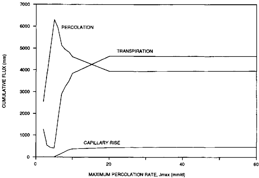
Fig. III.11 Sensitivity of DYNAMITE simulations of transpiration, capillary rise and percolation to uncertainty in the maximum percolation rate ( J_{max} ) using hydrologic input data for Kabo, Suriname.
