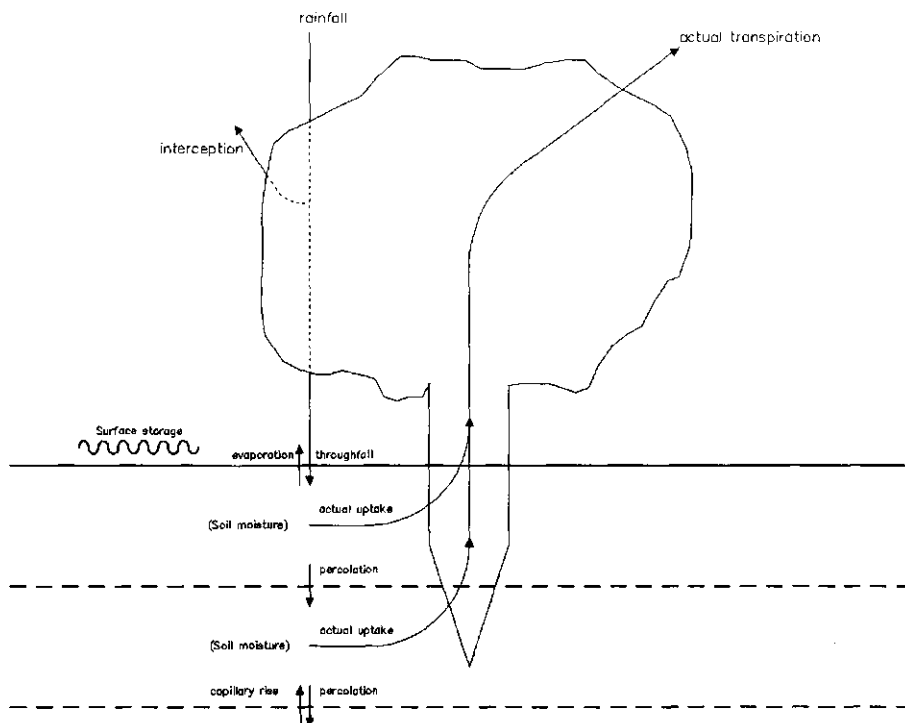
Fig. III.2 Schematic representation of the water balance sub-model in DYNAMITE.
