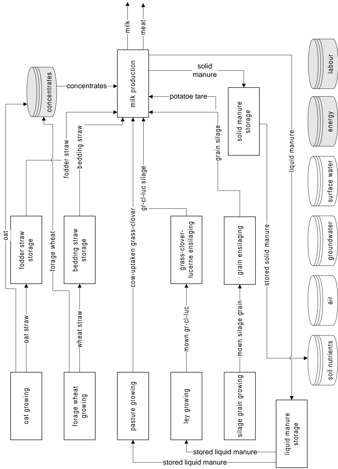
Figure 3. An example of a production line (milk production) modelled in terms of product flows. Rectangles represent process units. Drums represent internal (transparent) and external (grey) resources. Only main product flows are shown.
