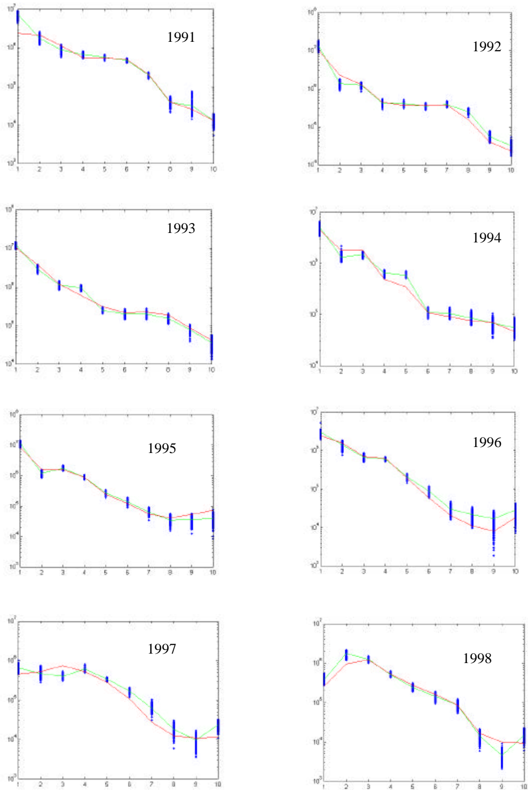
Figure 2. North Sea herring catch in number at age (wr+1) from 1991 to 1998, showing WG catch (red), bootstrap mean catch (green) and bootstrap values (blue) for catch scaled to biomass of landings (Scb). For other methods (Scn and Miss) mean numbers at age for WG are equal to mean numbers at age in the bootstrap.
