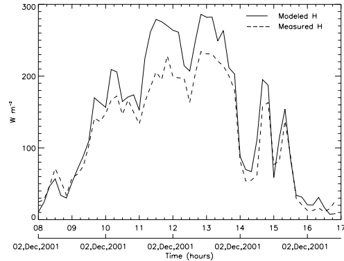
Figure 1. Reference modeled and measured sensible heat flux H for a cloudy day (2nd of Dec.) in Tamale.
