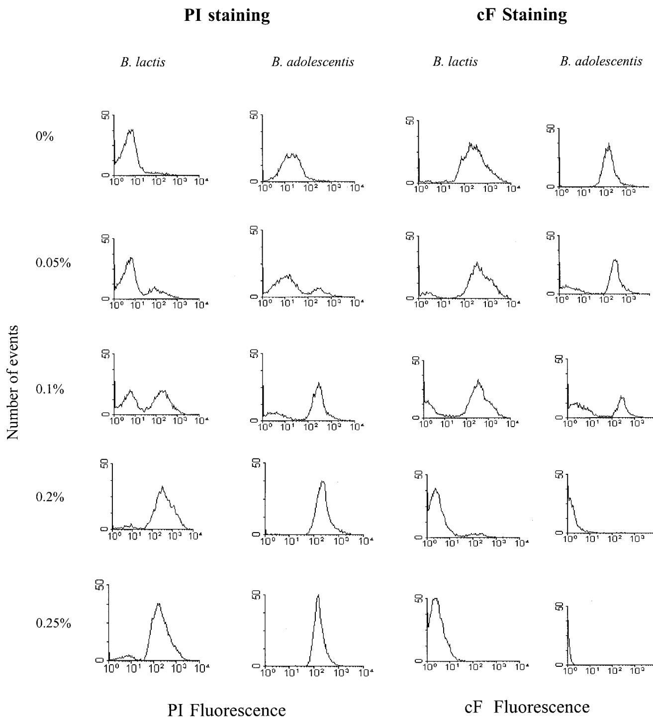
FIG. 3. Fluorescence histograms of B. lactis and B. adolescentis stained with 5 \mu g of PI/ml or 10 \mu M cFDA following exposure to different concentrations of dBS.
