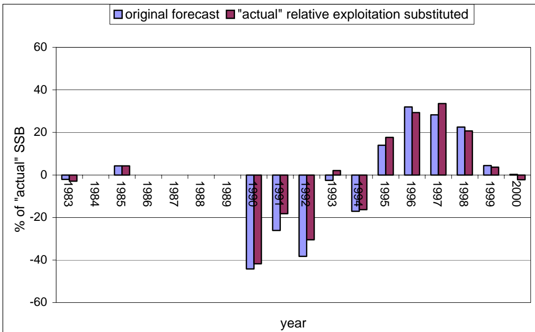
Figure 18. North Sea sole. Prediction errors in SSB surviving the current year in the original forecasts with status quo F assumption, and when the "actual" relative exploitation-at-age is substituted.
