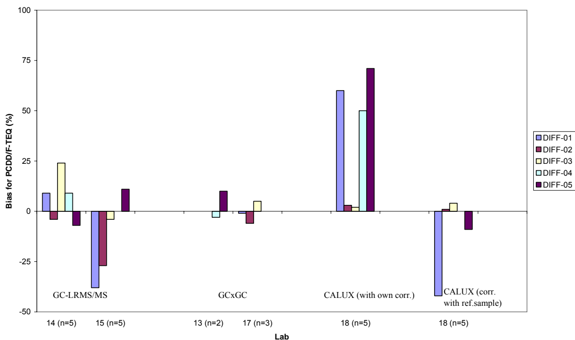
Figure 12. Bias for PCDD/F-TEQ obtained with various screening methods. The labnumbers are mentioned on the x-axis (together with the number of repetitions).
