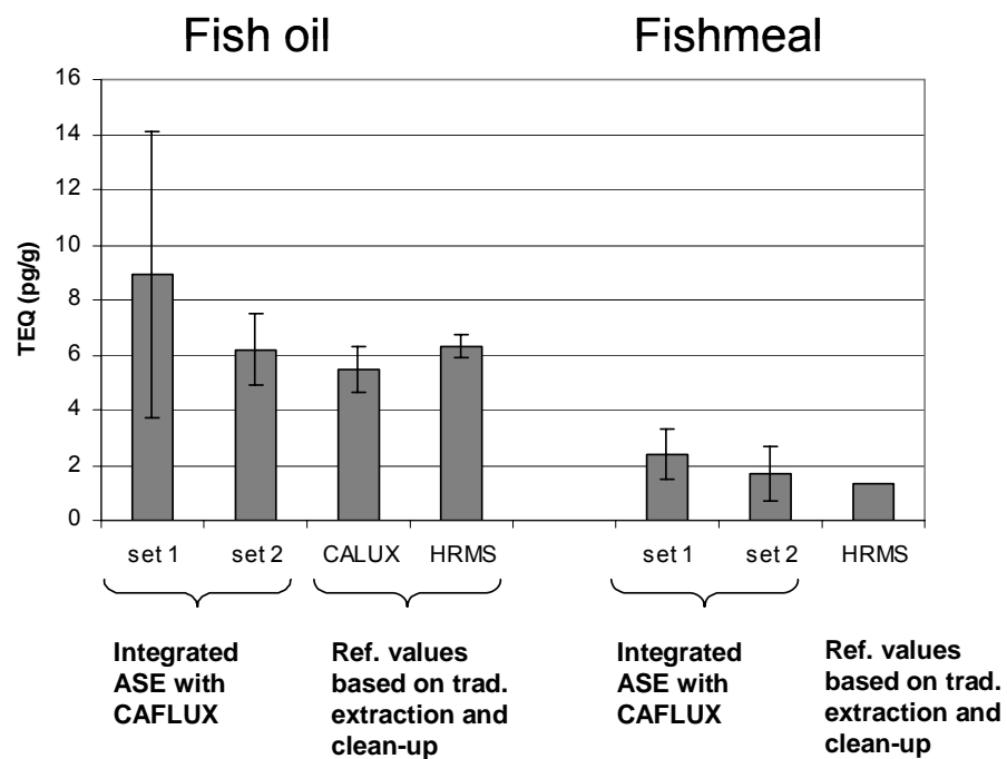
Figure 24. Dioxin content (pg TEQ/g sample) in fish oil and fishmeal determined with different methods. Set 1 and set 2 refer to analyses based on extractions with ASE followed by CALUX ( n = 3 ). The CALUX and HRMS values (lower bound TEQs) for the fish oil were produced within the EU DIFFERENCE project based on traditional extraction and clean-up procedures ( n = 6 ). For the fishmeal, the HRMS values (lower bound TEQs) are based on traditional extraction and clean-up procedures ( n = 1 ) performed at Environmental Chemistry, Umeå University. Error bars correspond to one standard deviation ( n = 3 ). Data from Nording et al. (2005).
