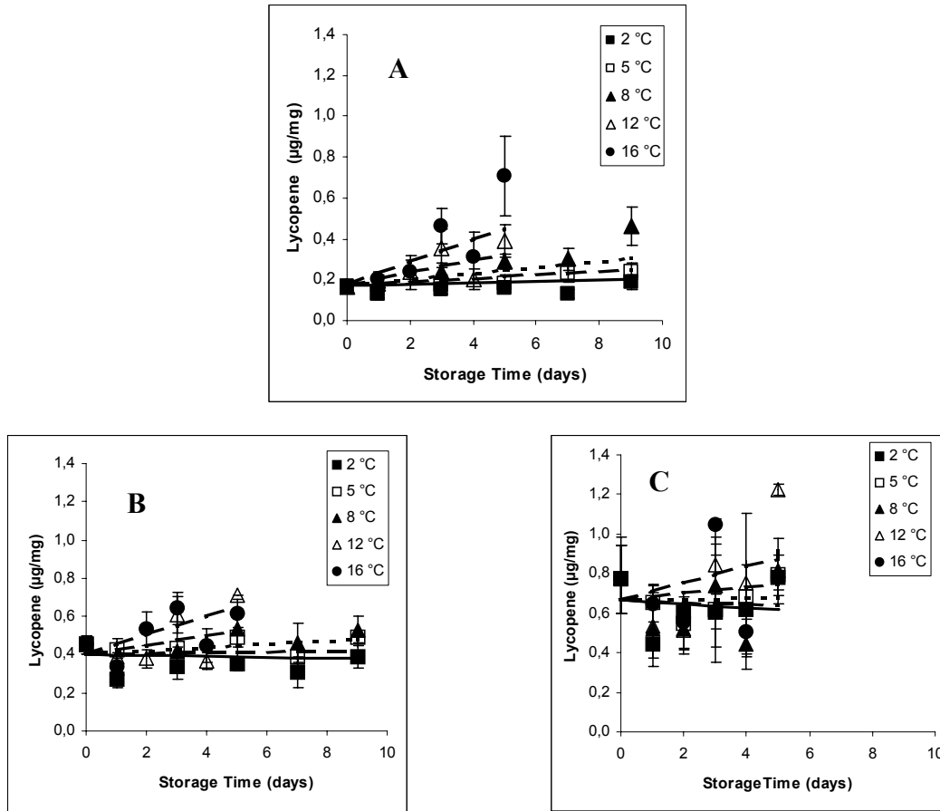
Fig. 2. Data and models fits of changes in lycopene concentration of fresh-cut tomato processed at stage I (A), stage II (B) and stage IV (C) during storage at different temperatures. Points are means + SD (n=5). Fit lines were obtained according to the kinetic model based upon pathway A.
