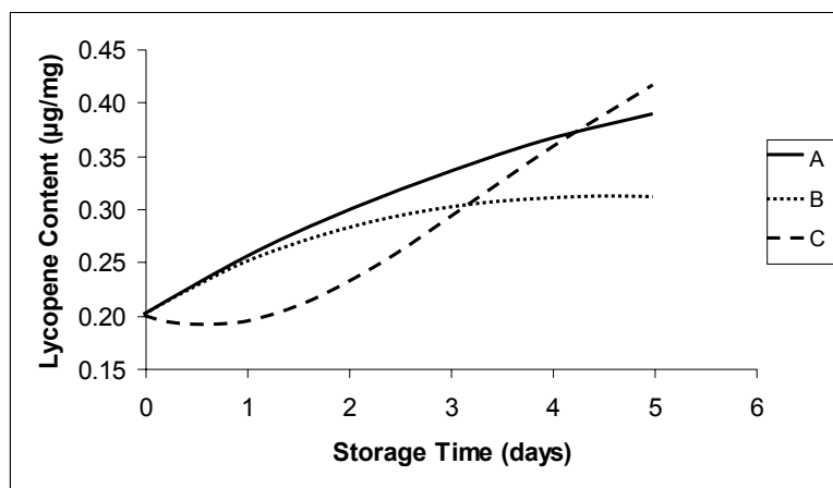
Fig. 3. Simulation of lycopene profiles in fresh-cut tomato slices during storage, using pathways A, B and C. (see text for details on pathways).
