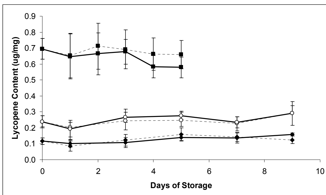
Fig. 1. Changes in lycopene concentration of sliced (dotted line) and intact tomato fruit (solid line) during storage at 5°C, when harvested at stages I (breaker) - ♦, II (pink) - ○, and IV (light red) ■.
