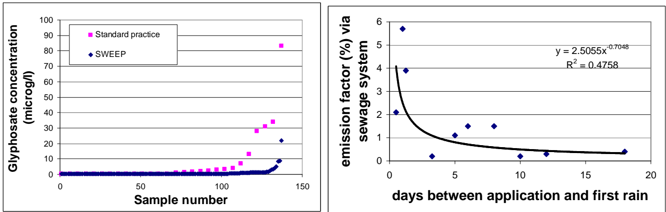
Figure 3A and 3B. Glyphosate in surface water at discharge points in samples taken at moments of rain events after herbicide application on pavements (A, left), and relation between rain fall in test quarters and emission via the sewage water system (B, right) in study areas in 2002, 2003 and 2004.
