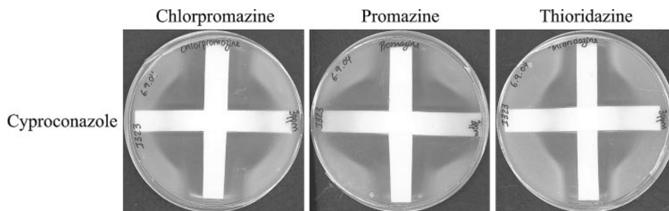
FIG. 1. Synergistic activity between cyproconazole and the putative modulators of ABC transporter activity chlorpromazine, promazine, and thioridazine against growth of M. graminicola strain IPO323 in crossed-paper-strip experiments. The horizontal strips were impregnated with cyproconazole (1 mg liter -1 in methanol), and the vertical strips were impregnated with the modulators (3,000 mg liter -1 in methanol).
