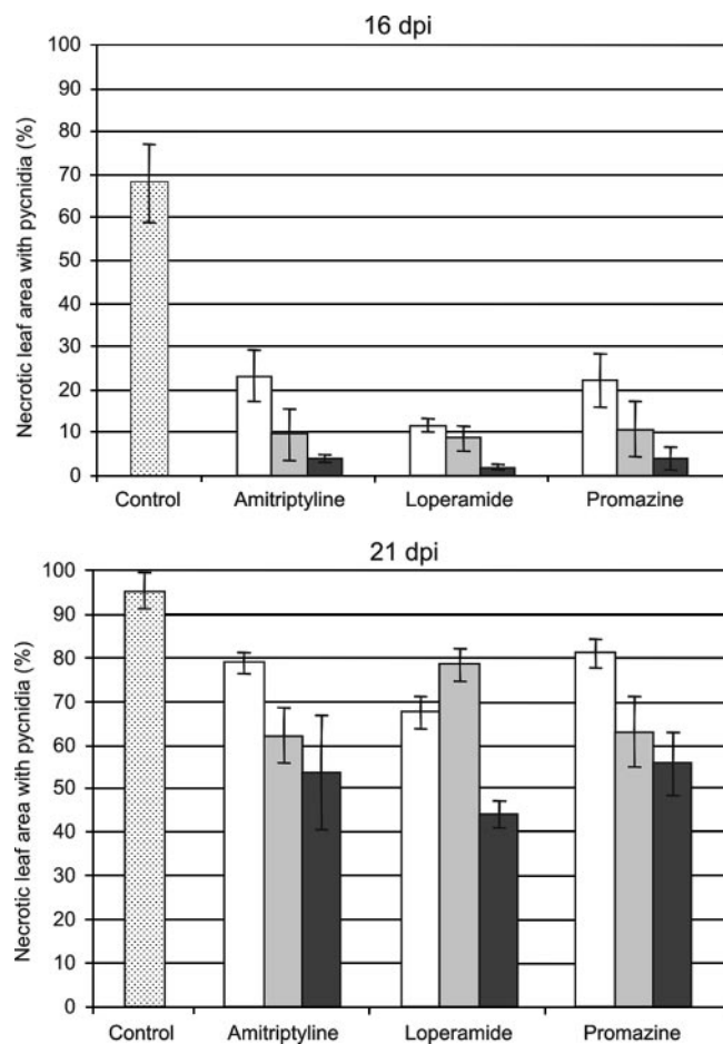
FIG. 2. Activities of amitriptyline, loperamide, and promazine in control of M. graminicola IPO323 on cultivar Obelisk wheat seedlings in curative foliar spray tests. The concentrations of the compounds tested were 1 mg liter -1 (open bars), 10 mg liter -1 (gray bars), and 100 mg liter -1 (black bars). Disease was assessed at 16 and 21 dpi. The bars indicate the mean percentages of necrotic leaf area with pycnidia, and the error bars indicate standard deviations.
