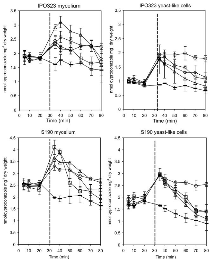
FIG. 3. Effects of modulators on accumulation of [ ^{14}\text{C} ]cyproconazole ( 100\ \mu\text{M} ) by mycelium and yeast-like cells of M. graminicola IPO323 and S190. The modulators ( 300\ \mu\text{M} ) amitriptyline ( \square ), chlorpromazine ( \circ ), flavanone ( \triangle ), and promazine ( \diamond ) were added 30 min after the addition of cyproconazole (dashed line). —, control treatment. The error bars indicate the standard deviations of the means.
