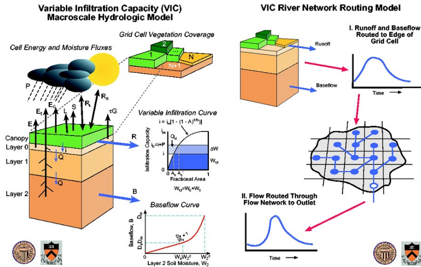
Fig 2. Schematic representation of the main features of the VIC model (left) and the routing algorithm (right). Graphs are taken from the VIC-website: http://www.hydro.washington.edu/Lettenmaier/Models/VIC/VIChome.html .
