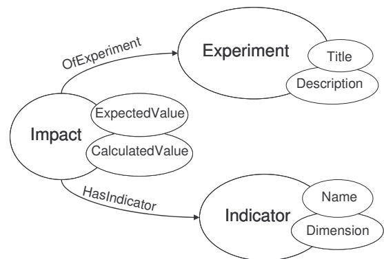
Figure 3. An ontology snapshot showing the concepts ‘Impact’, ‘Indicator’ and ‘Experiment’ (large circles), their relationships (arrows) and their data-properties (small circles).
