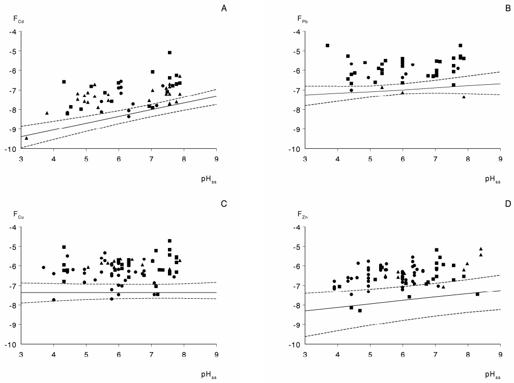
Fig. 3 Plots of F against pH_{ss} for cadmium (A), lead (B), copper (C) and zinc (D). Triangles: Toxicity endpoints for plants; circles: toxicity endpoints for invertebrates; squares: toxicity endpoints for microbial processes. Solid line: median critical limit function (50% confidence); dotted lines: critical limit functions with 90% confidence. (5% and 95%)
